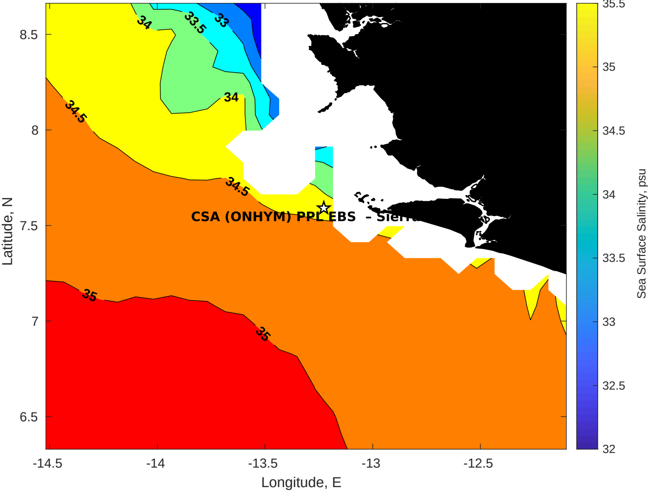
Surface Salinity for CSA (ONHYM) PPL EBS - Sierra Leone at 06-Aug-2025 00:00:00
