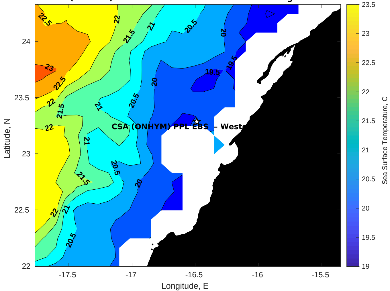
SST for CSA (ONHYM) PPL EBS - Western Sahara at 06-Aug-2025 00:00:00
