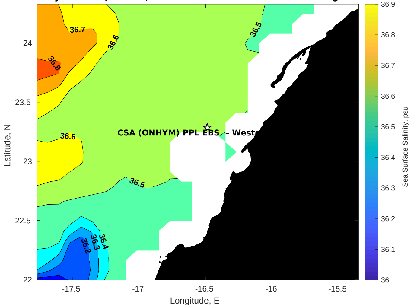
Surface Salinity for CSA (ONHYM) PPL EBS - Western Sahara at 06-Aug-2025 00:00:00
