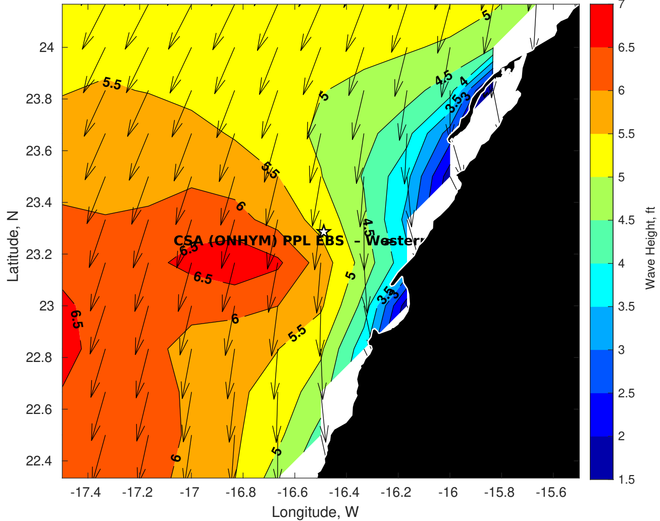
Wave Height (ft) for CSA (ONHYM) PPL EBS - Western Sahara at 07-Aug-2025 09:00:00
