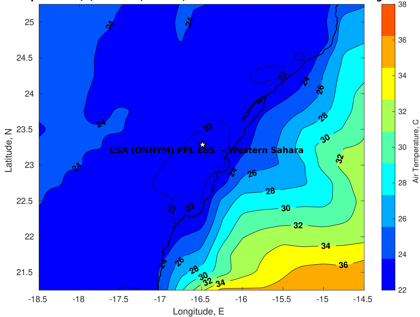
Air Temperature (C) for CSA (ONHYM) PPL EBS - Western Sahara at 07-Aug-2025
