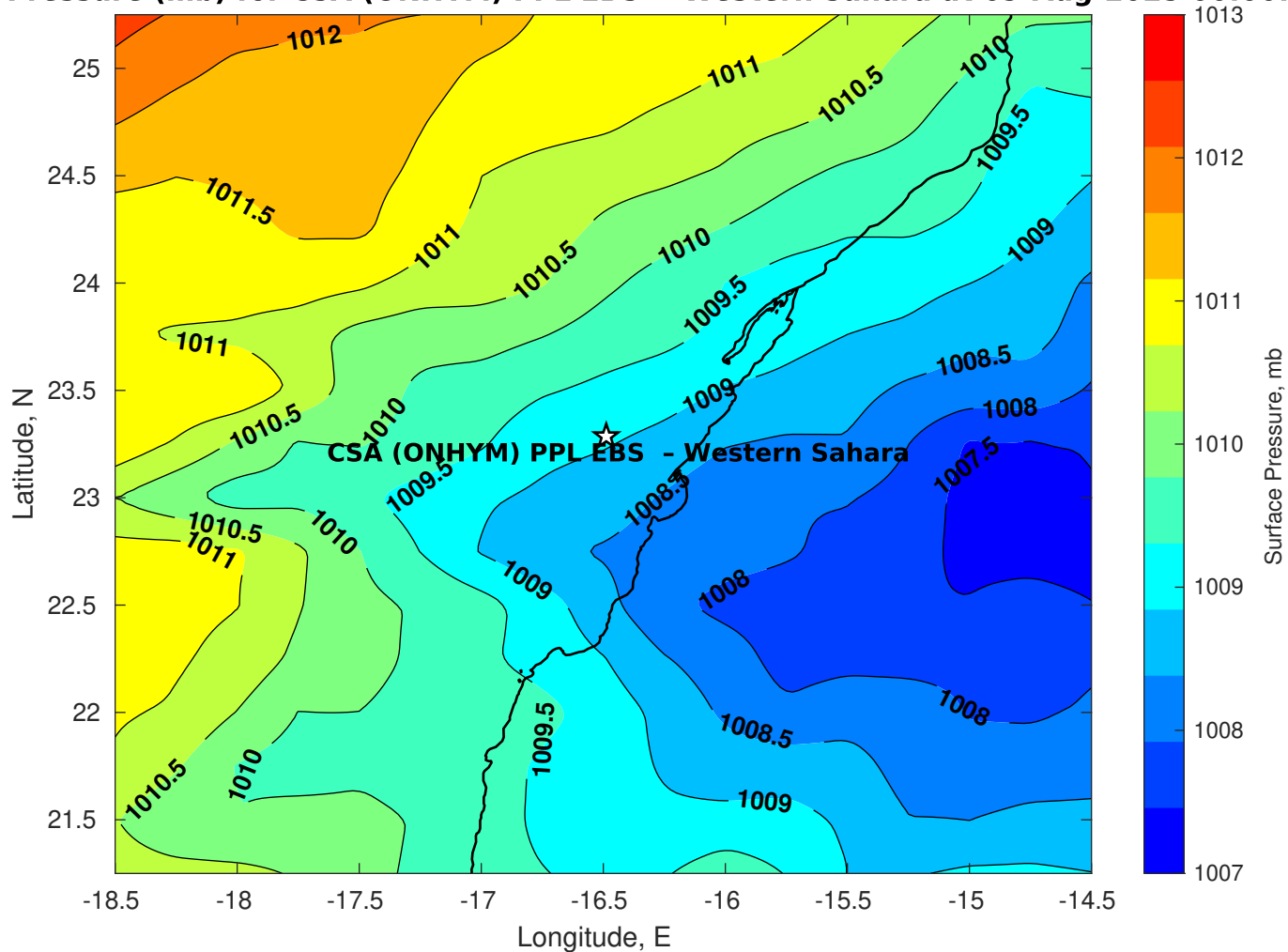
Surface Pressure (mb) for CSA (ONHYM) PPL EBS - Western Sahara at 09-Aug-2025 00:00:00
