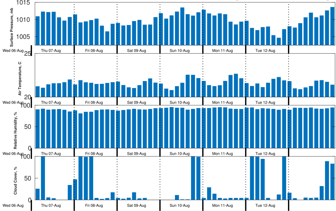
Met Forecast for CSA (ONHYM) PPL EBS - Western Sahara from 07-Aug-2025 00:00:00 to 14-Aug-2025 00:00:00
