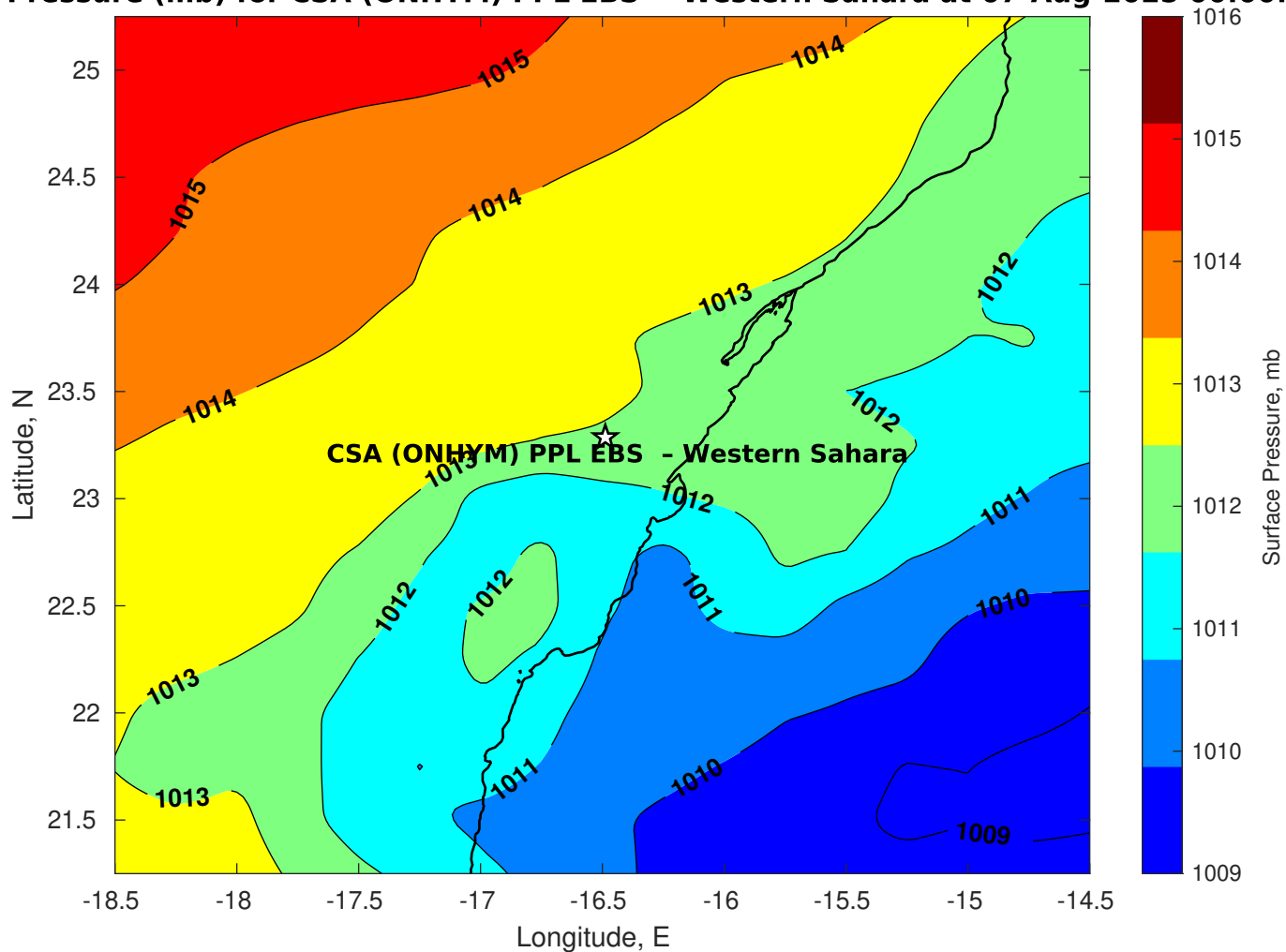
Surface Pressure (mb) for CSA (ONHYM) PPL EBS - Western Sahara at 07-Aug-2025 00:00:00
