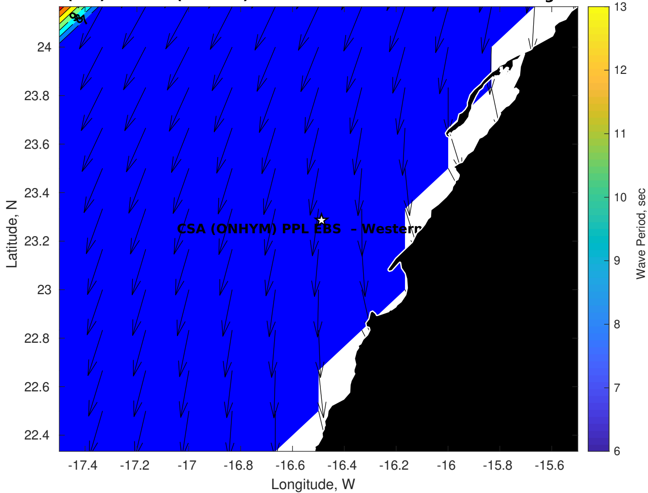
Wave Period (sec) for CSA (ONHYM) PPL EBS - Western Sahara at 07-Aug-2025 09:00:00
