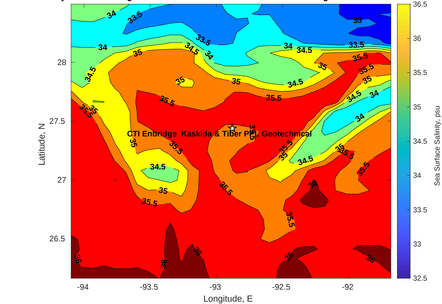
Surface Salinity for CTI Enbridge Kaskida & Tiber PPL Geotechnical at 06-Aug-2025 00:00:00
