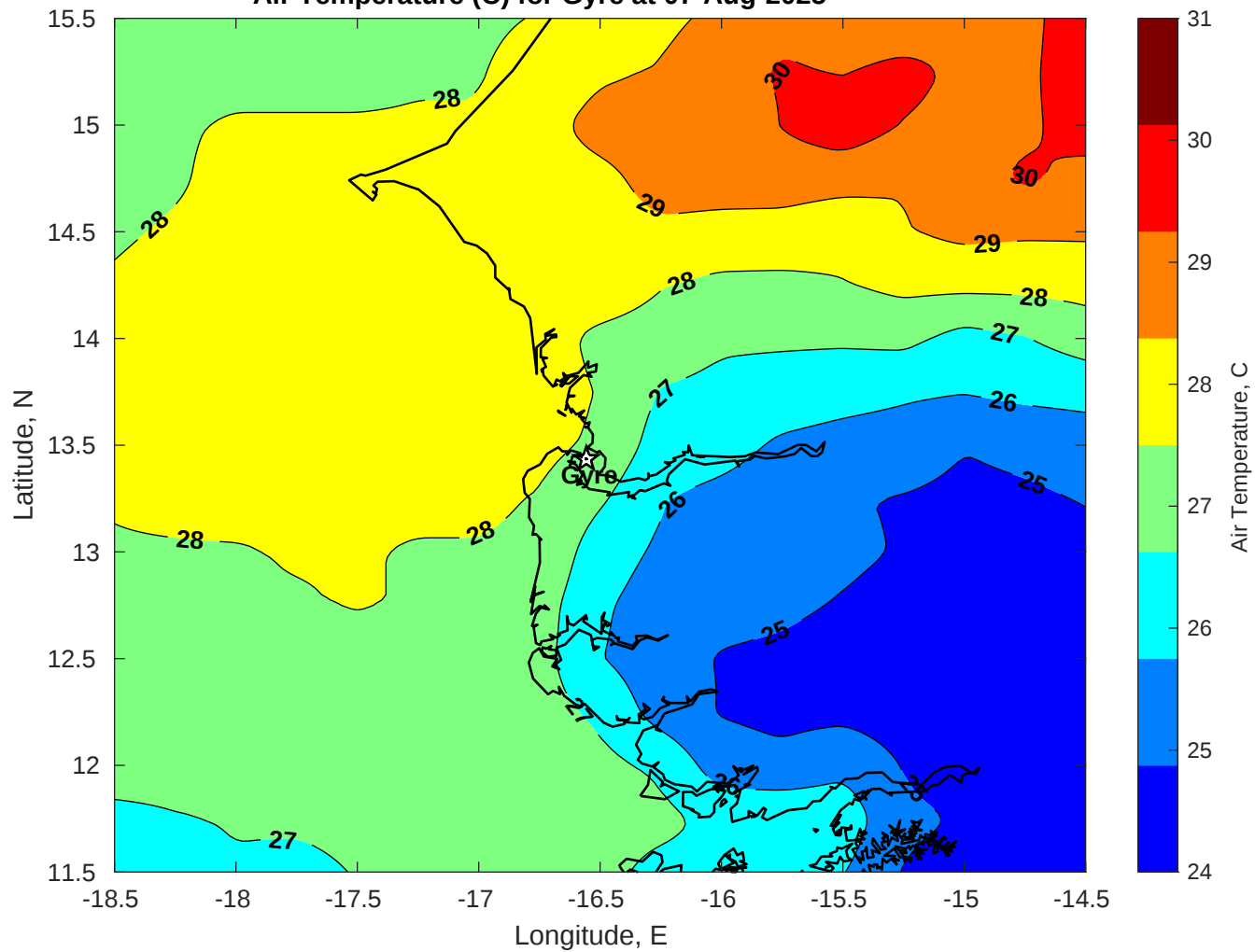
Air Temperature (C) for Gyre at 07-Aug-2025
