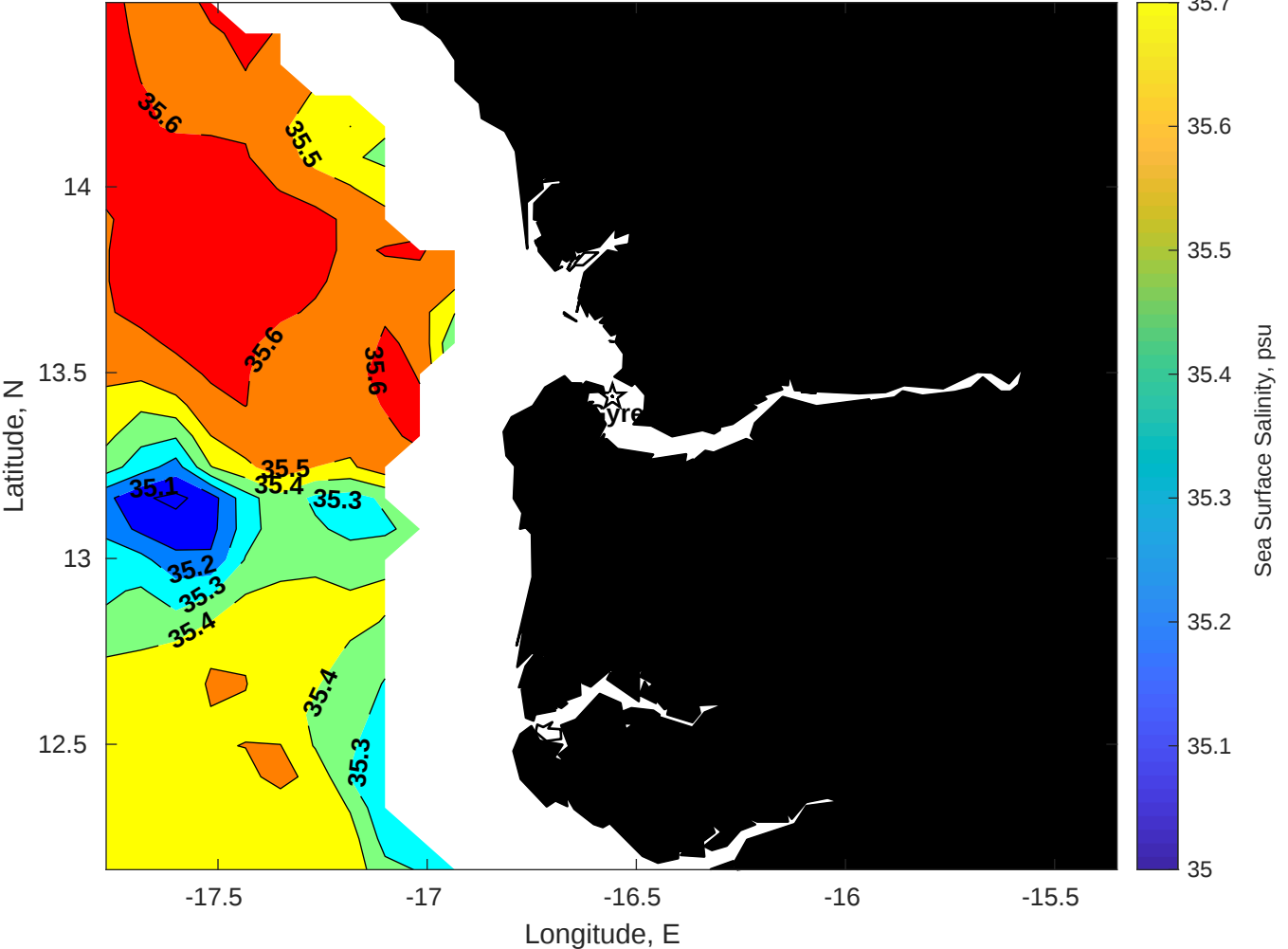
Surface Salinity for Gyre at 06-Aug-2025 00:00:00
