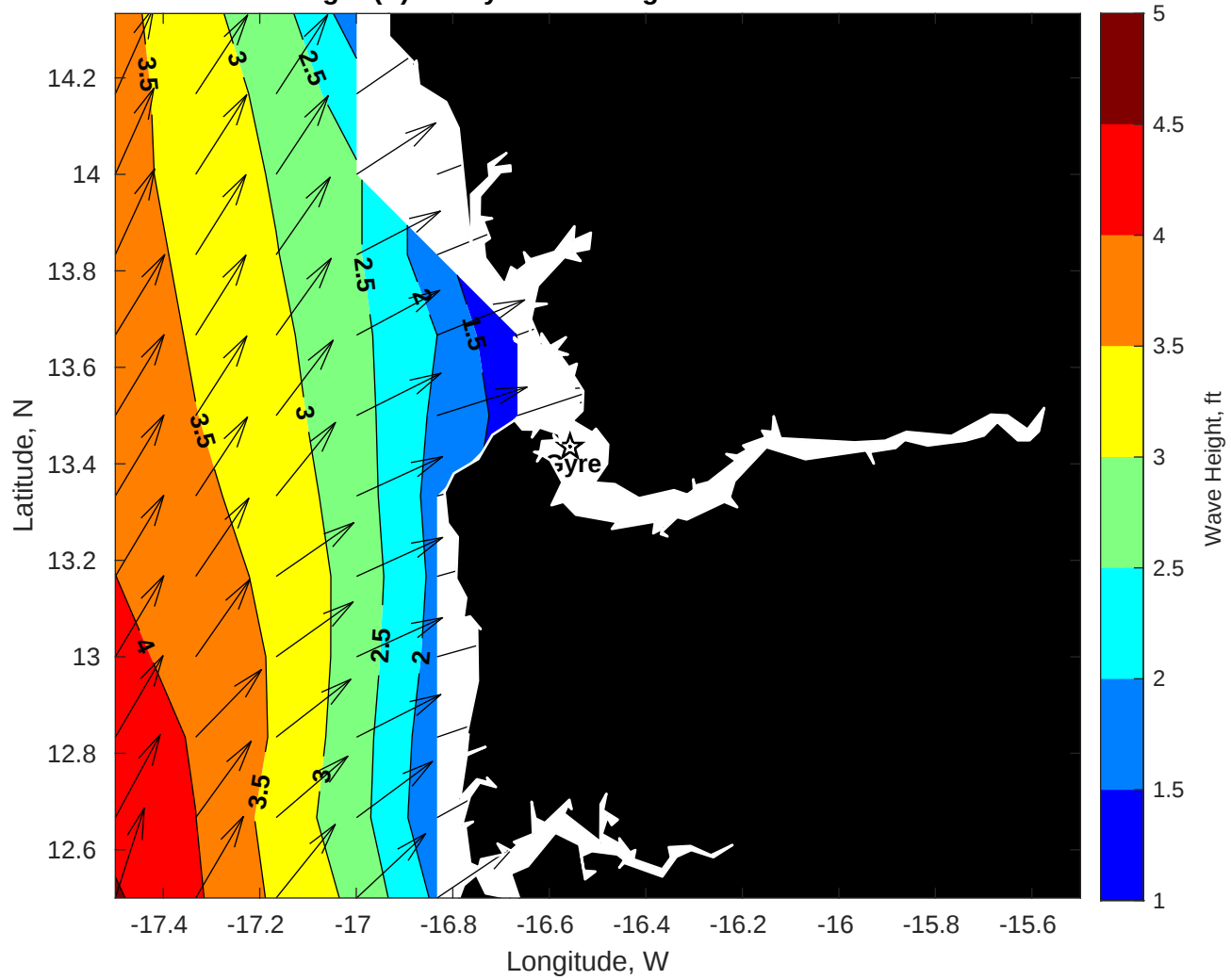
Wave Height (ft) for Gyre at 07-Aug-2025 09:00:00
