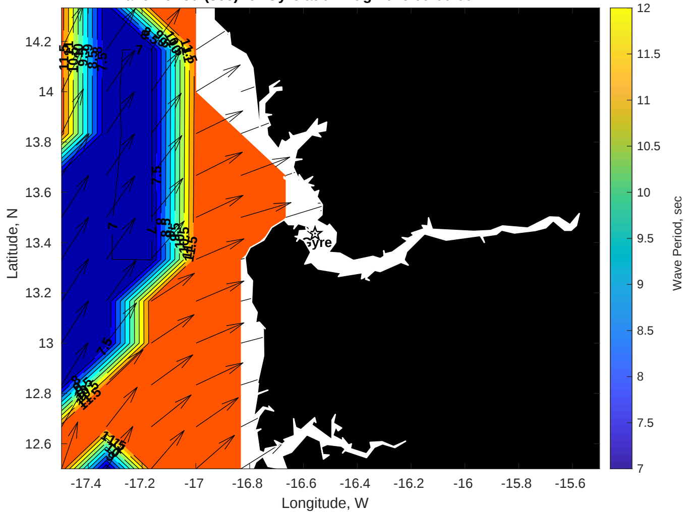
Wave Period (sec) for Gyre at 07-Aug-2025 09:00:00
