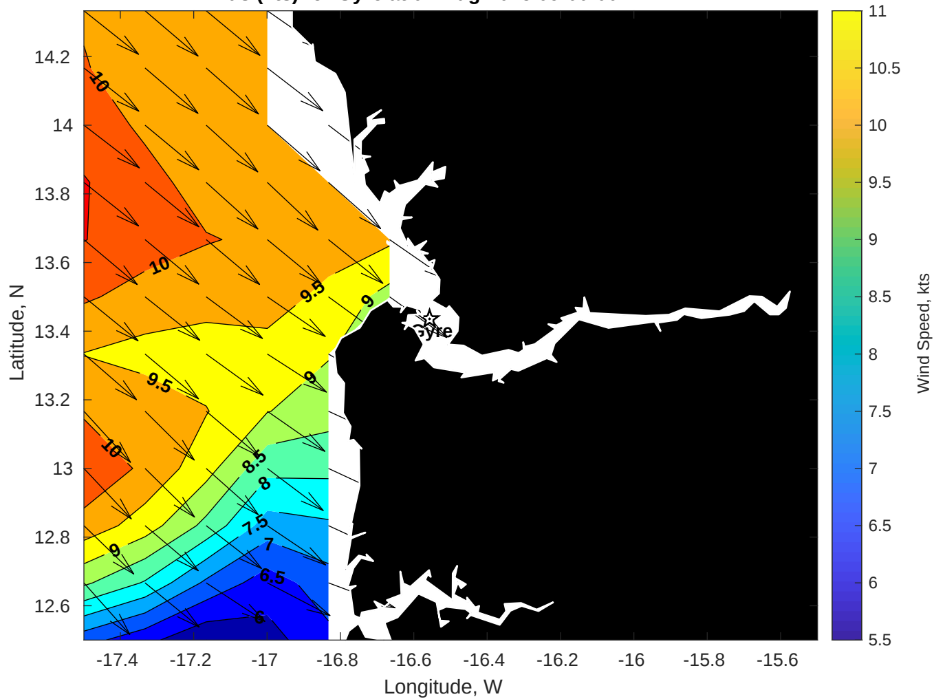
Winds (kts) for Gyre at 07-Aug-2025 09:00:00
