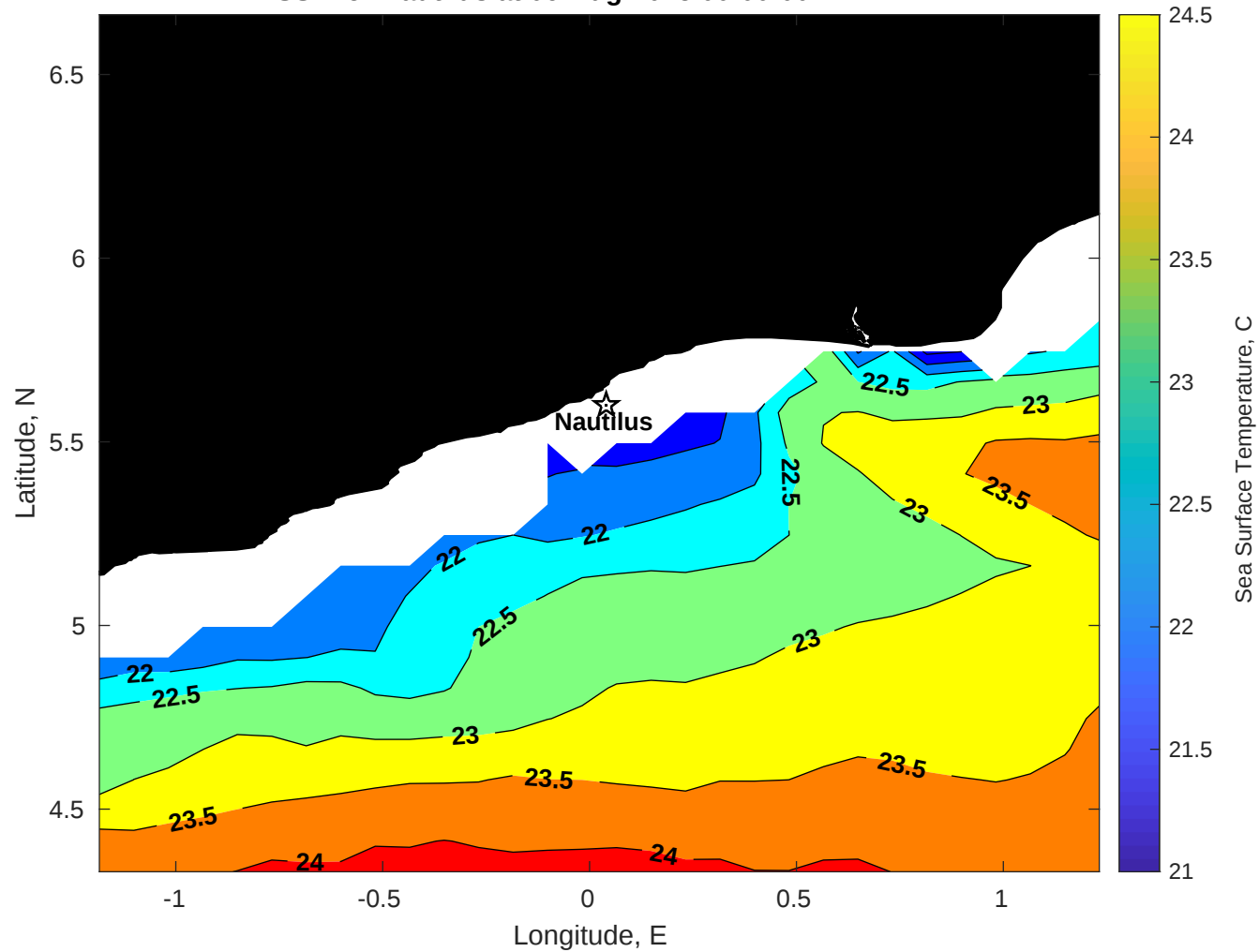
SST for Nautilus at 06-Aug-2025 00:00:00
