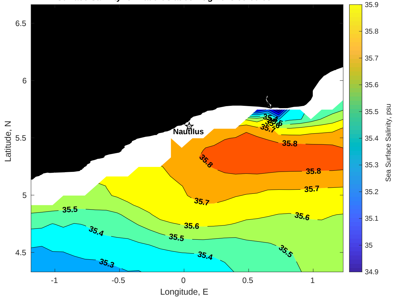
Surface Salinity for Nautilus at 06-Aug-2025 00:00:00
