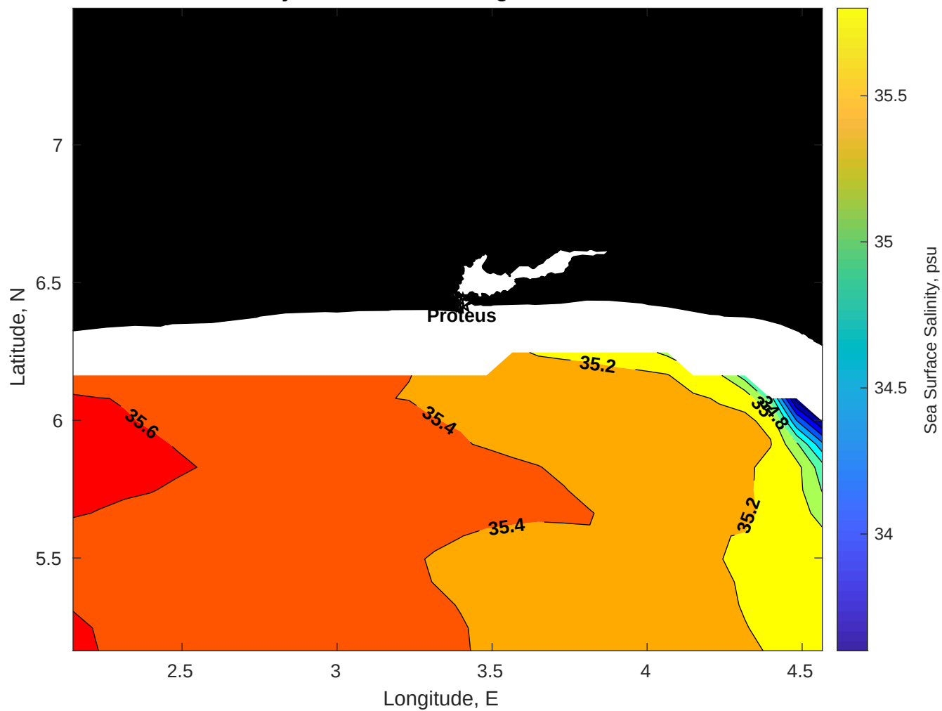
Surface Salinity for Proteus at 06-Aug-2025 00:00:00
