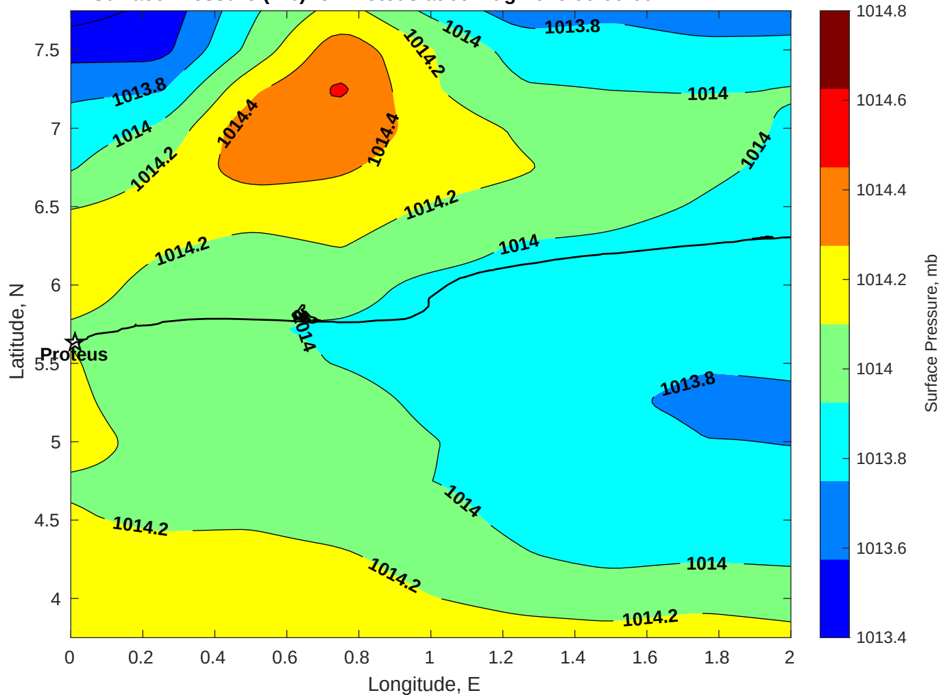
Surface Pressure (mb) for Proteus at 09-Aug-2025 00:00:00
