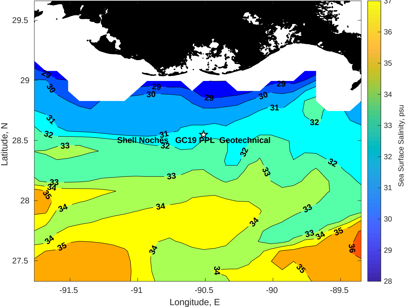
Surface Salinity for Shell Noches GC19 PPL Geotechnical at 06-Aug-2025 00:00:00
