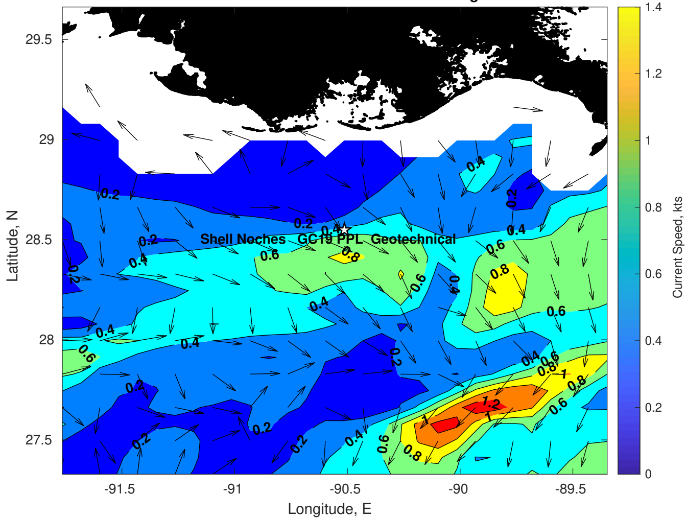
Surface Currents for Shell Noches GC19 PPL Geotechnical at 06-Aug-2025 00:00:00
