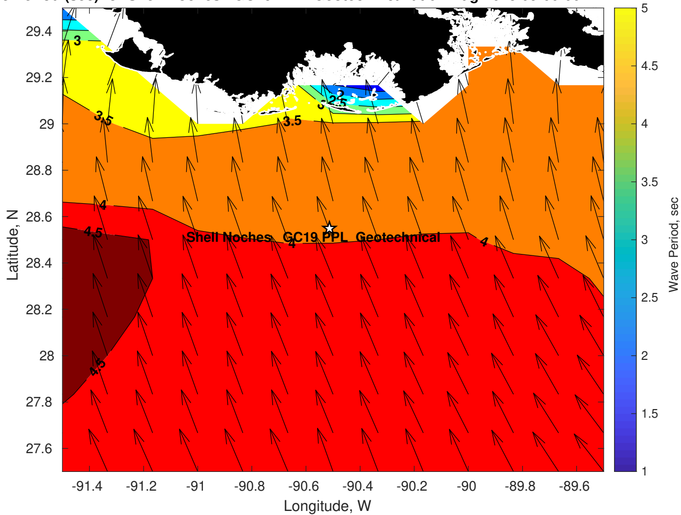
Wave Period (sec) for Shell Noches GC19 PPL Geotechnical at 07-Aug-2025 09:00:00
