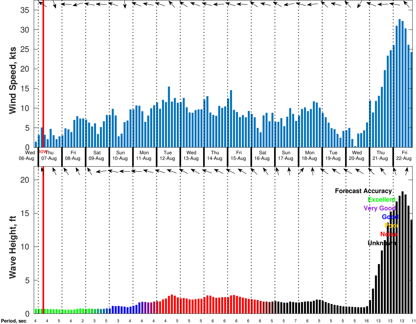
Wind & Wave Forecast for Shell Noches GC19 PPL Geotechnical from 06-Aug-2025 20:00:00 to 22-Aug-2025 20:00:00
