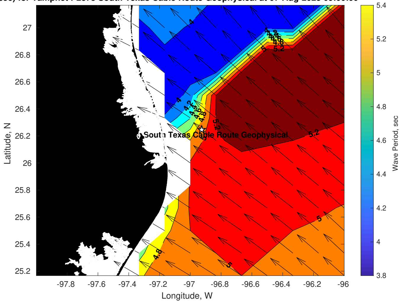
Period (sec) for Tampnet P2378 South Texas Cable Route Geophysical at 07-Aug-2025 09:00:00
