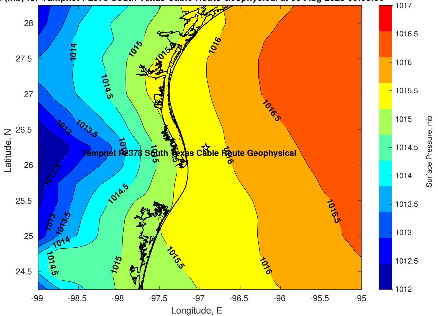
Pressure (mb) for Tampnet P2378 South Texas Cable Route Geophysical at 08-Aug-2025 00:00:00
