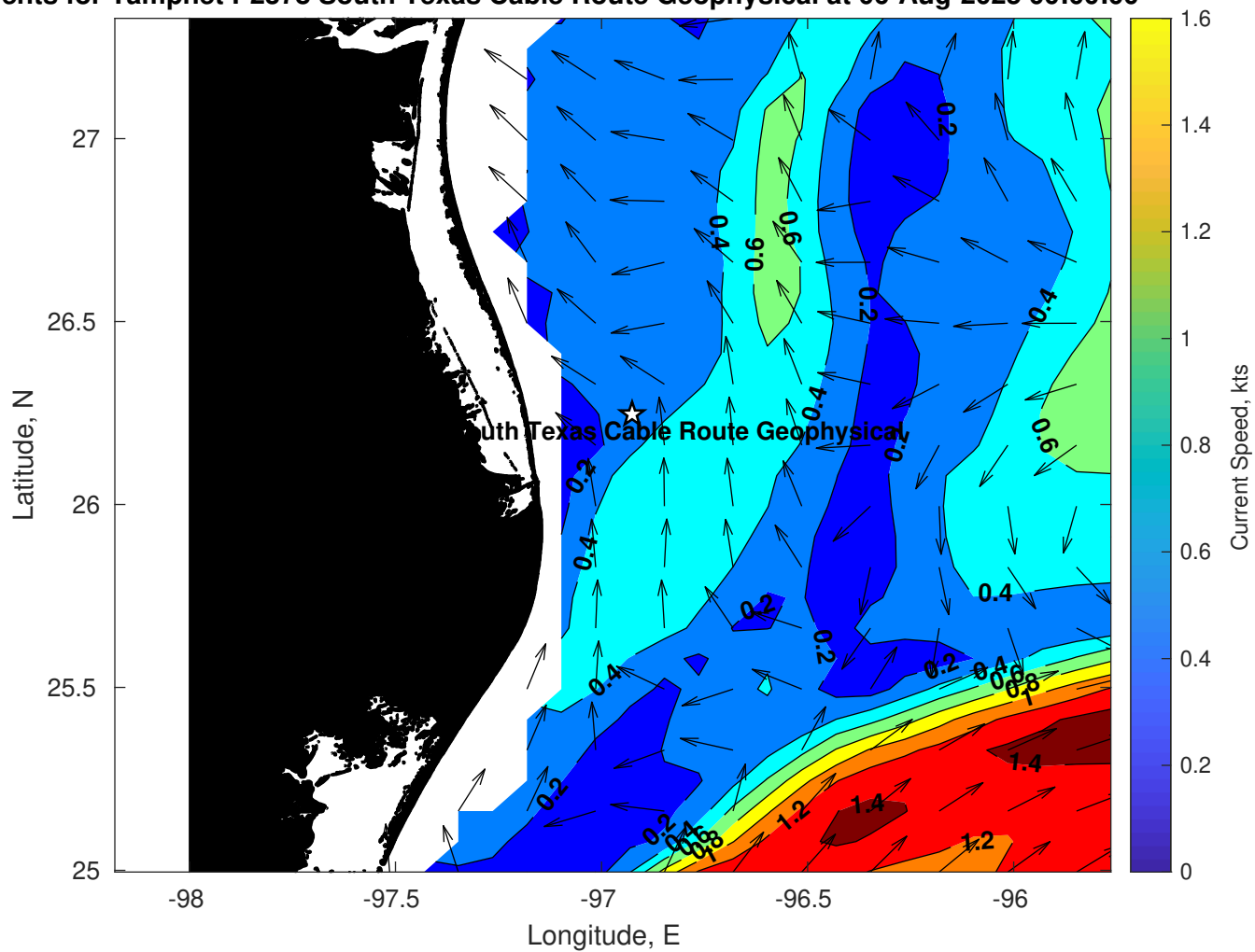
Surface Currents for Tampnet P2378 South Texas Cable Route Geophysical at 06-Aug-2025 00:00:00
