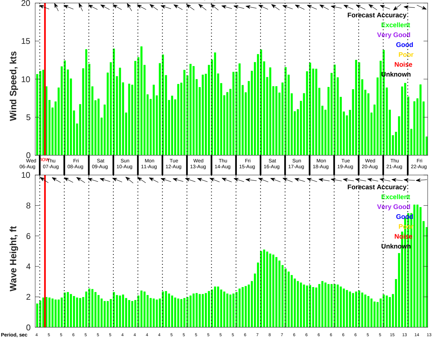
Wind & Wave Forecast for Tampnet P2378 South Texas Cable Route Geophysical from 06-Aug-2025 20:00:00 to 22-Aug-2025 20:00:00
