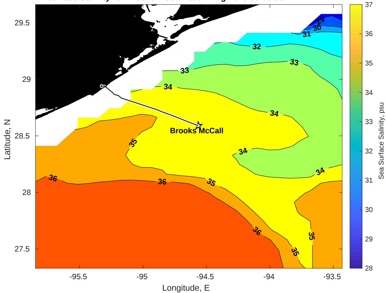
Surface Salinity for Brooks McCall at 07-Aug-2025 00:00:00
