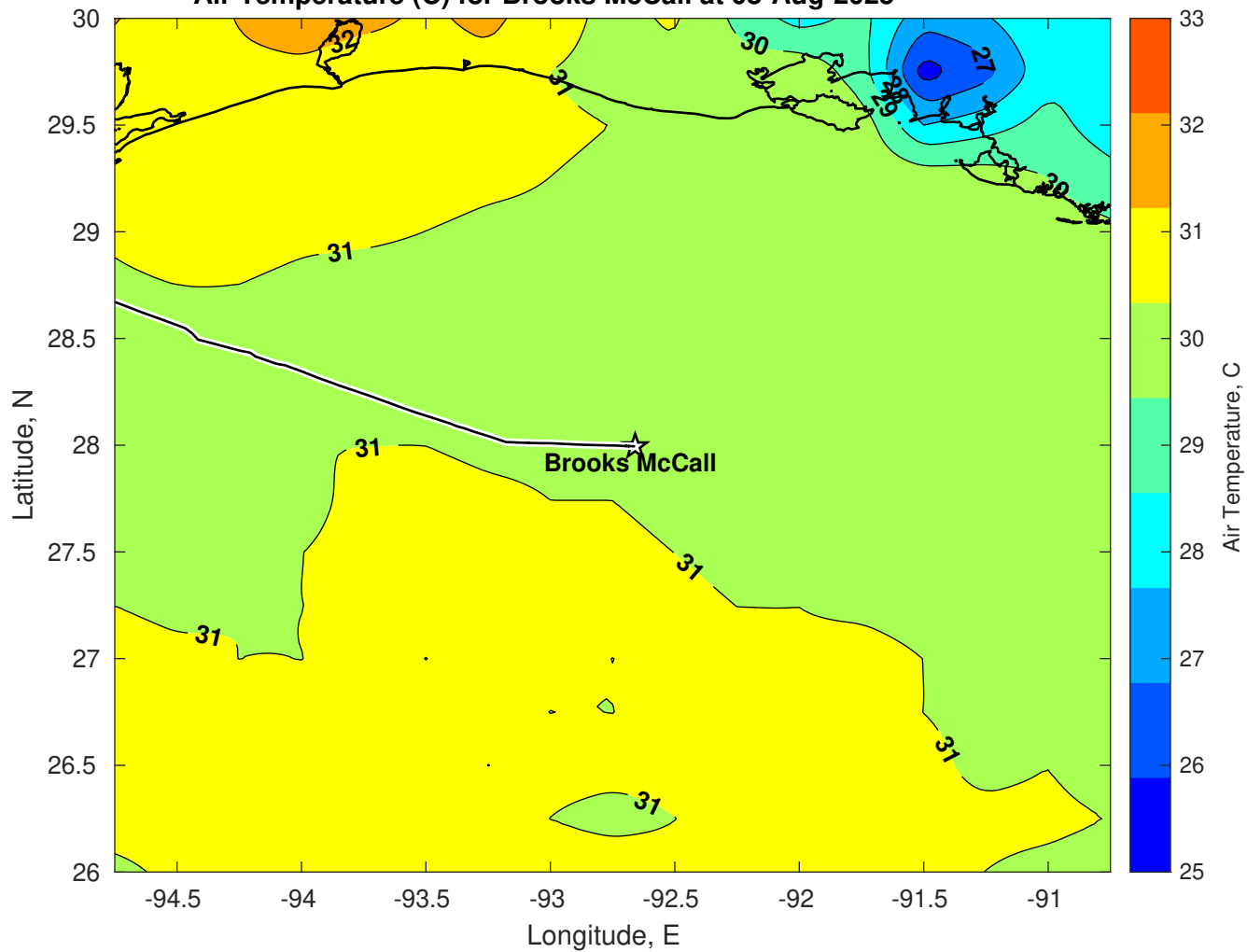
Air Temperature (C) for Brooks McCall at 08-Aug-2025
