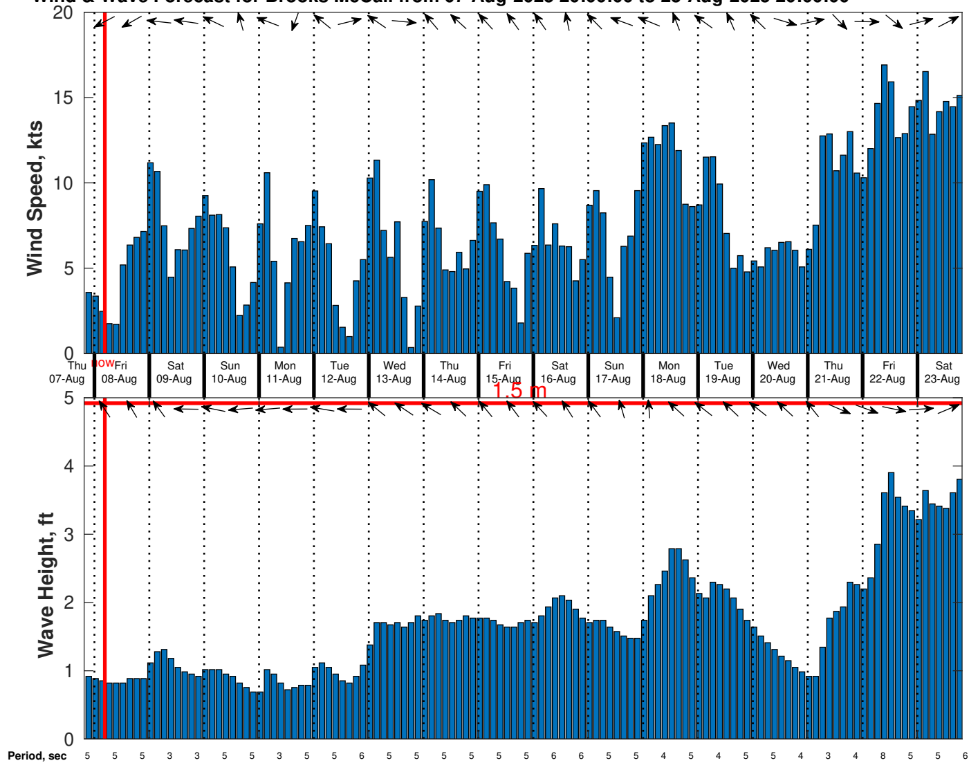
Wind & Wave Forecast for Brooks McCall from 07-Aug-2025 20:00:00 to 23-Aug-2025 20:00:00
