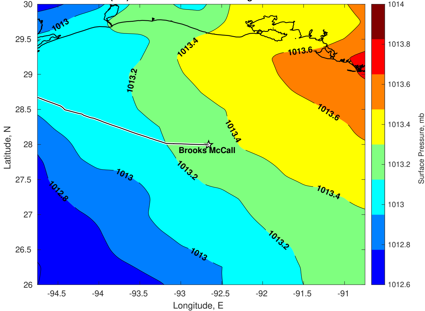
Surface Pressure (mb) for Brooks McCall at 10-Aug-2025 00:00:00
