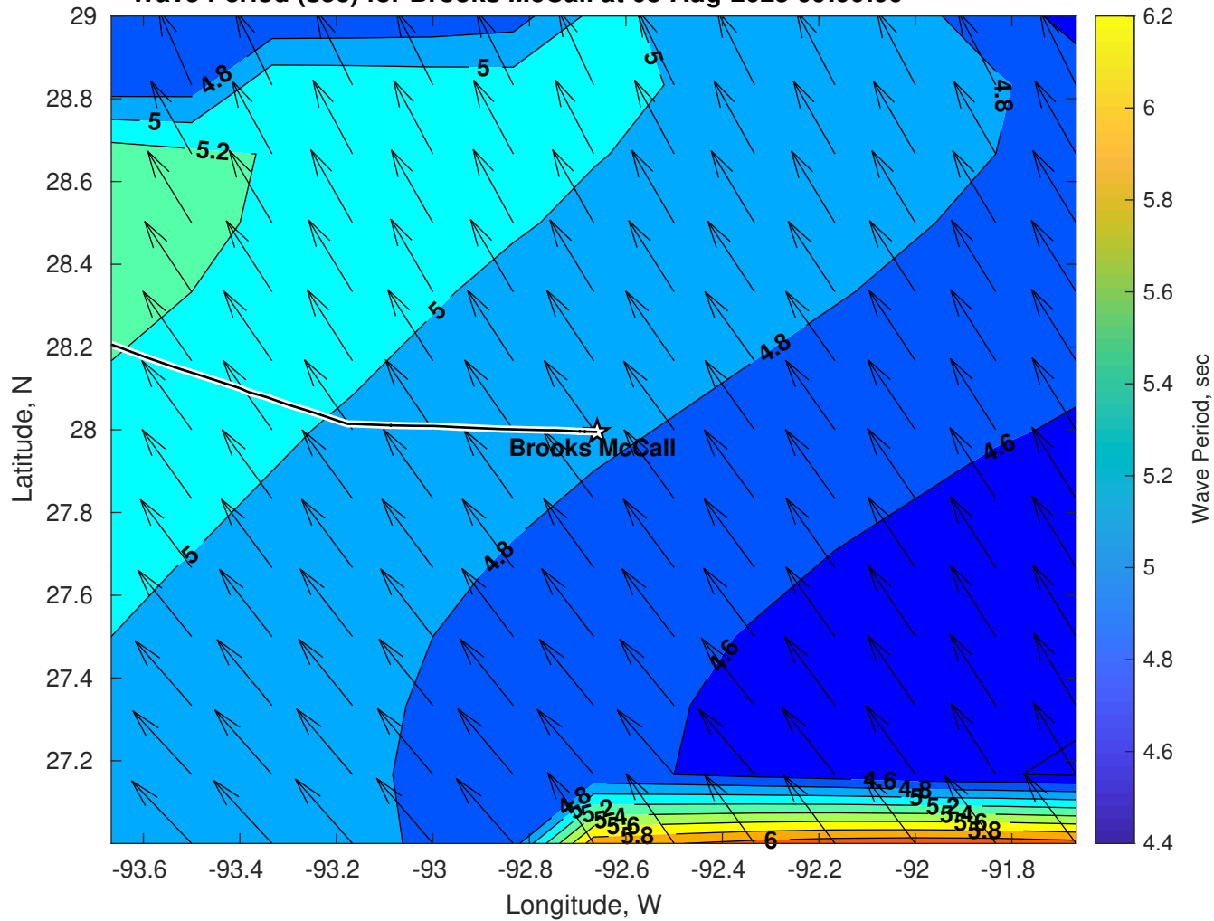
Wave Period (sec) for Brooks McCall at 08-Aug-2025 09:00:00
