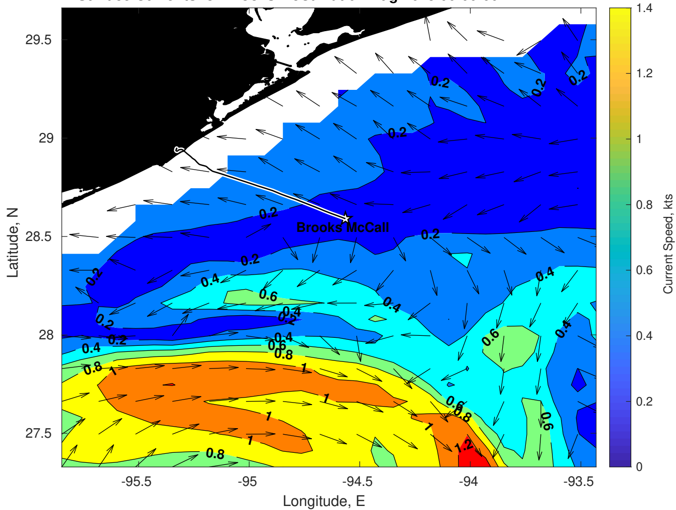
Surface Currents for Brooks McCall at 07-Aug-2025 00:00:00
