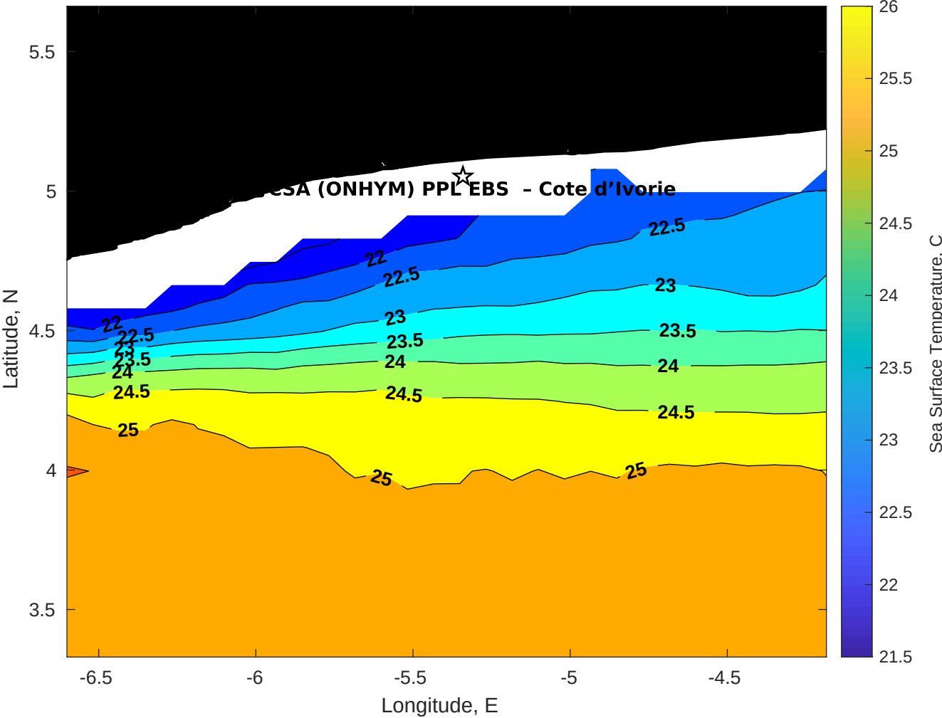
SST for CSA (ONHYM) PPL EBS - Cote d'Ivoire at 07-Aug-2025 00:00:00
