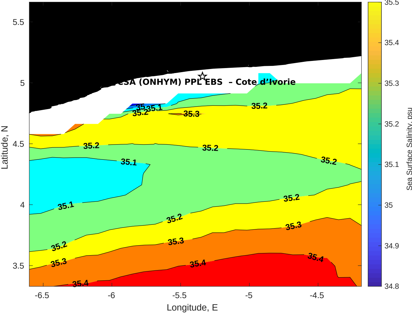
Surface Salinity for CSA (ONHYM) PPL EBS - Cote d'Ivoire at 07-Aug-2025 00:00:00
