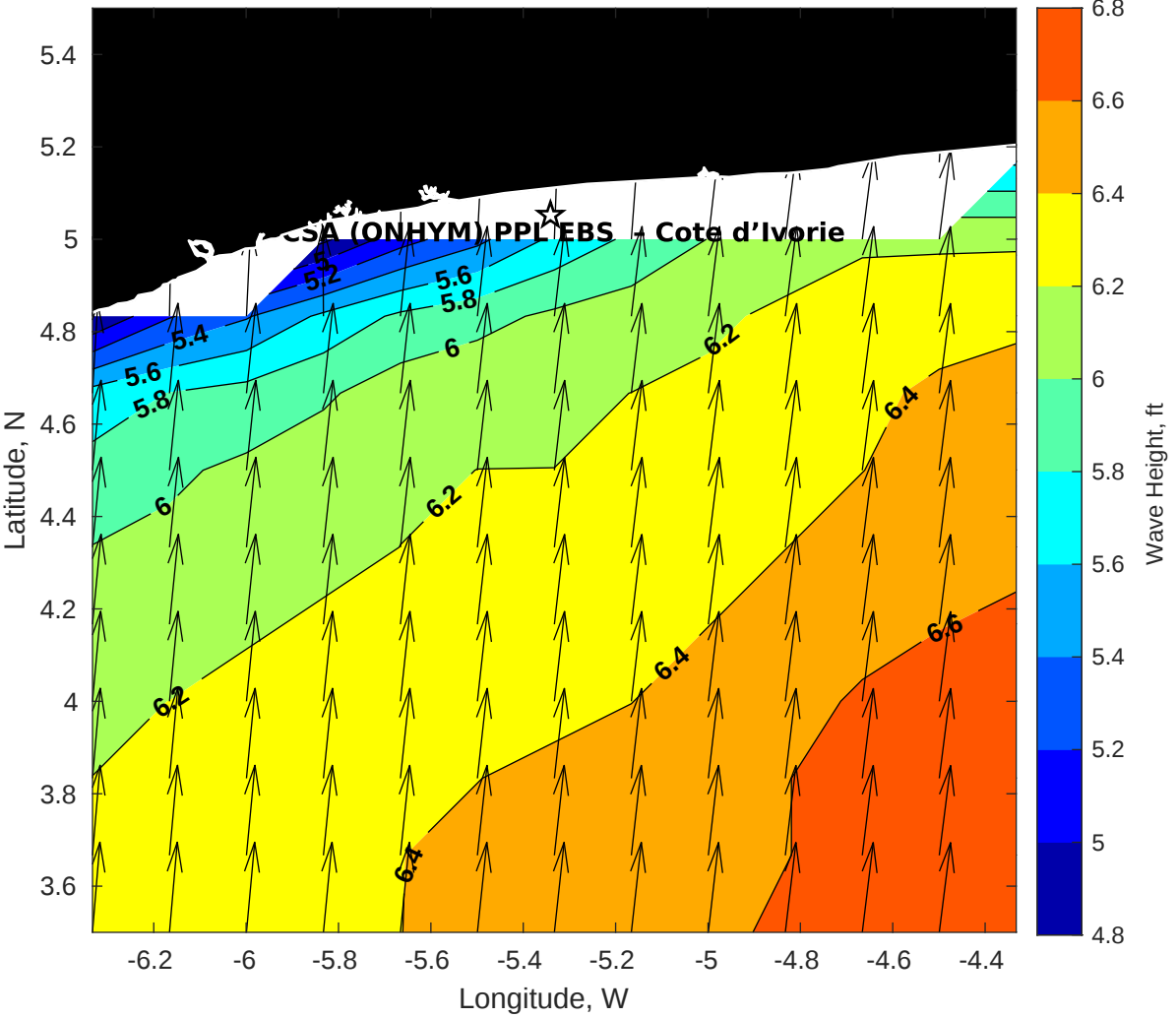
Wave Height (ft) for CSA (ONHYM) PPL EBS - Cote d'Ivoire at 08-Aug-2025 09:00:00
