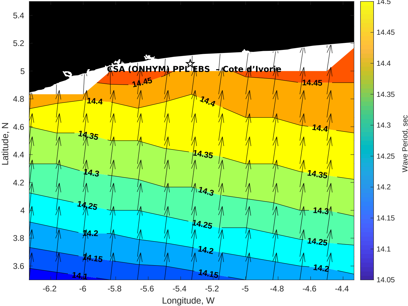
Wave Period (sec) for CSA (ONHYM) PPL EBS - Cote d'Ivoire at 08-Aug-2025 09:00:00
