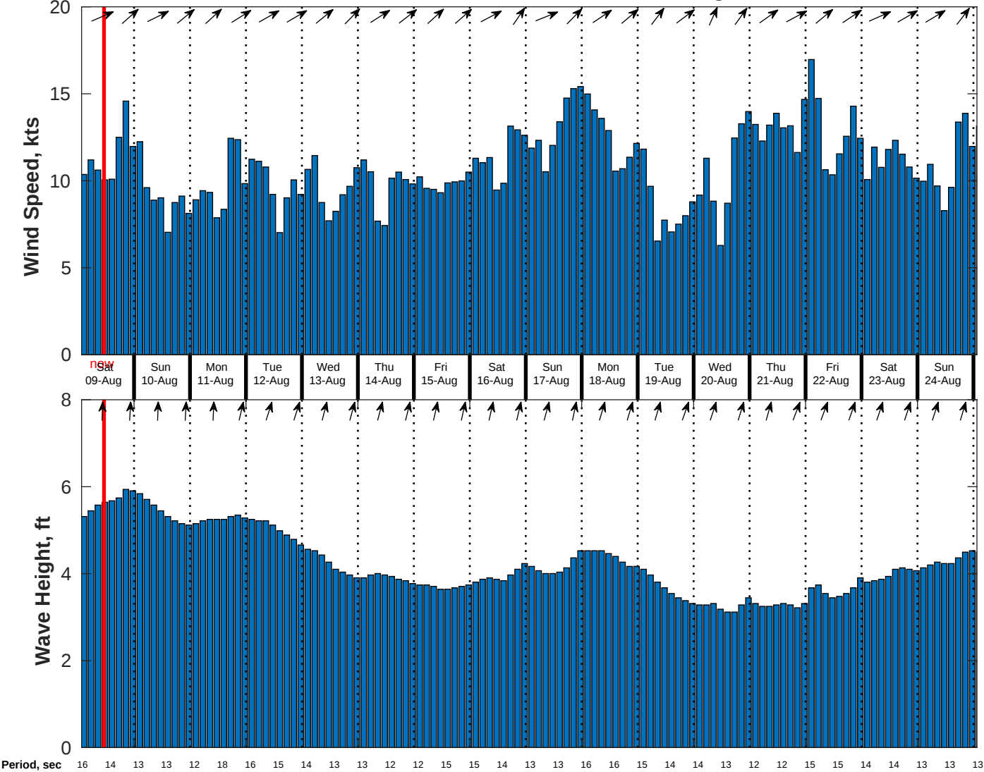
Wind & Wave Forecast for CSA (ONHYM) PPL EBS - Cote d'Ivoire from 08-Aug-2025 01:00:00 to 24-Aug-2025 01:00:00
