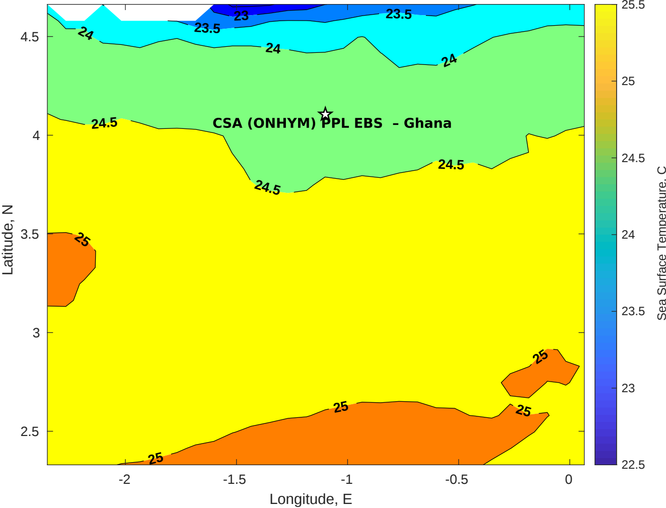
SST for CSA (ONHYM) PPL EBS - Ghana at 07-Aug-2025 00:00:00
