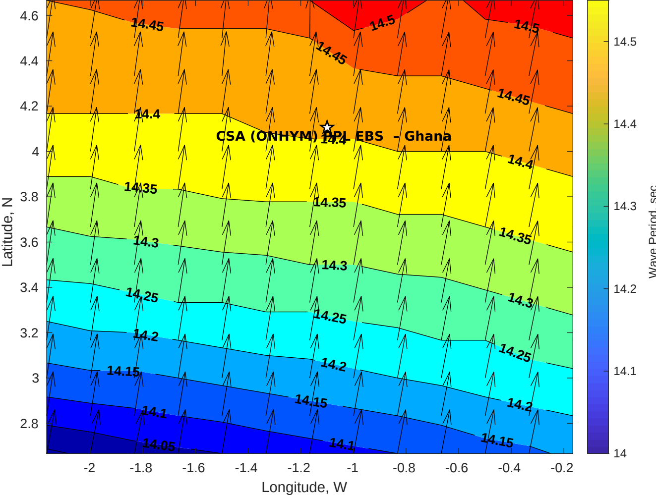
Wave Period (sec) for CSA (ONHYM) PPL EBS - Ghana at 08-Aug-2025 09:00:00
