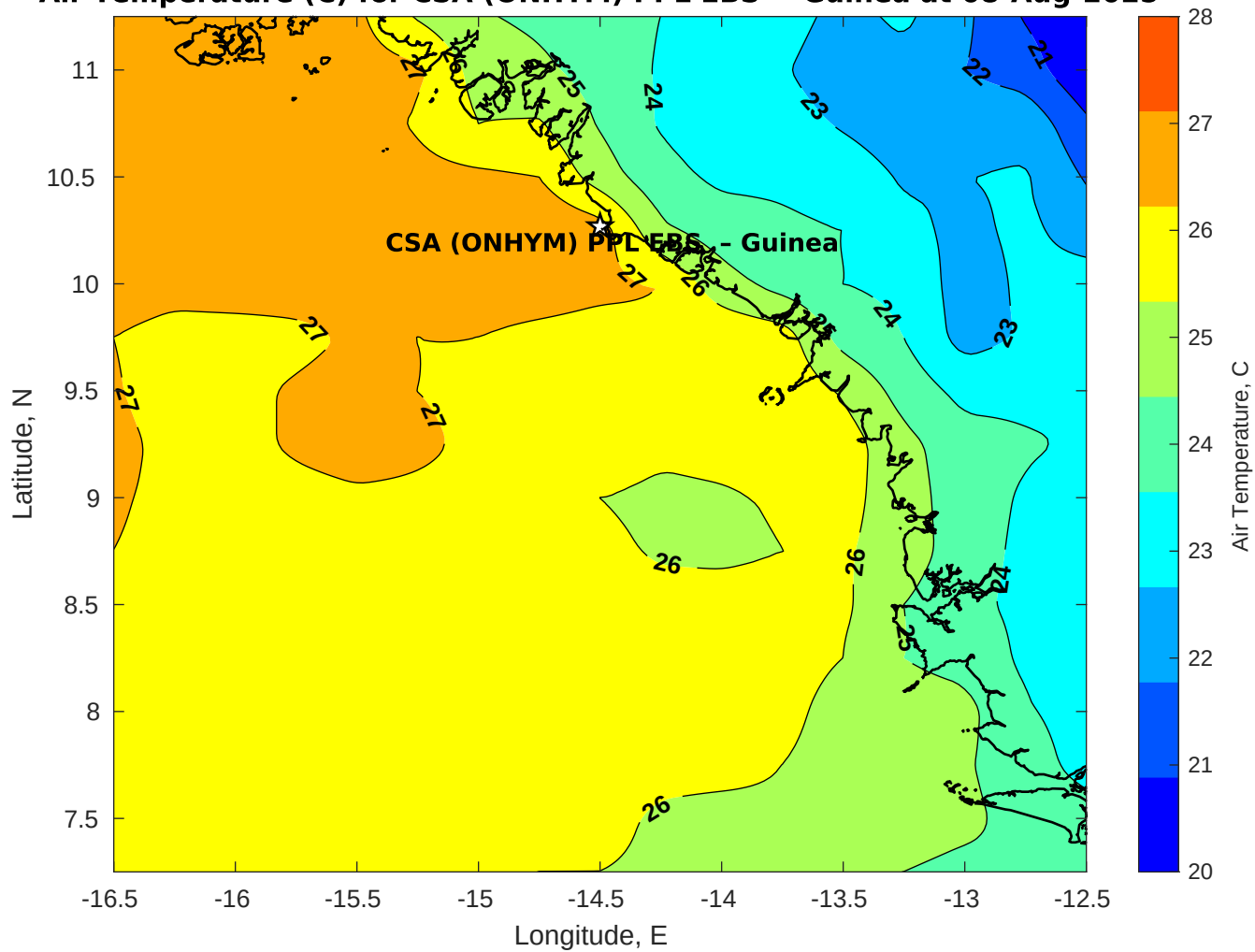
Air Temperature (C) for CSA (ONHYM) PPL EBS - Guinea at 08-Aug-2025
