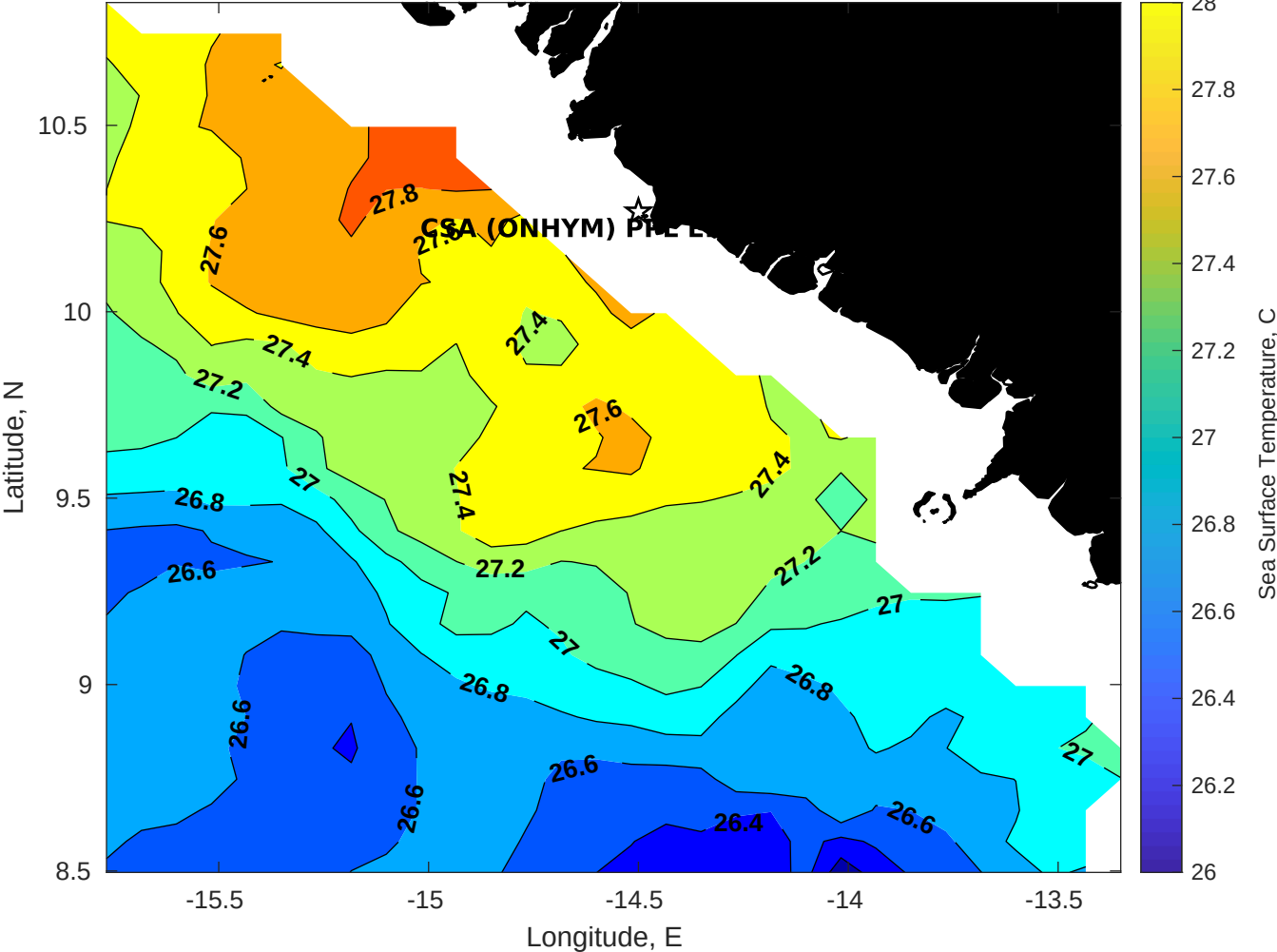
SST for CSA (ONHYM) PPL EBS - Guinea at 07-Aug-2025 00:00:00
