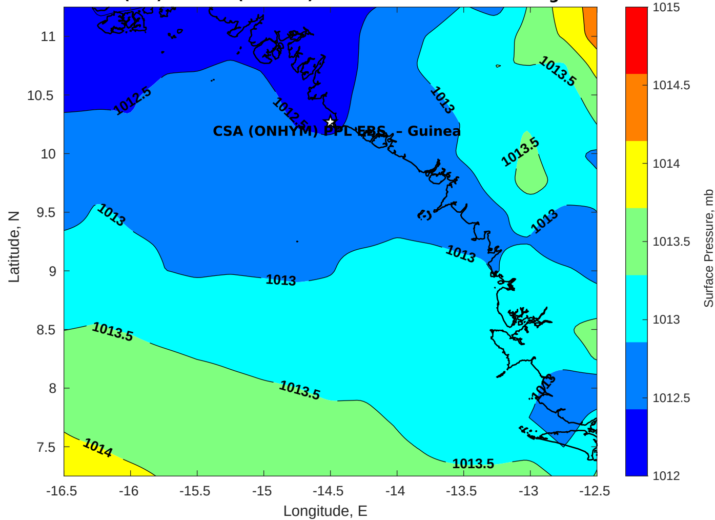
Surface Pressure (mb) for CSA (ONHYM) PPL EBS - Guinea at 08-Aug-2025 00:00:00
