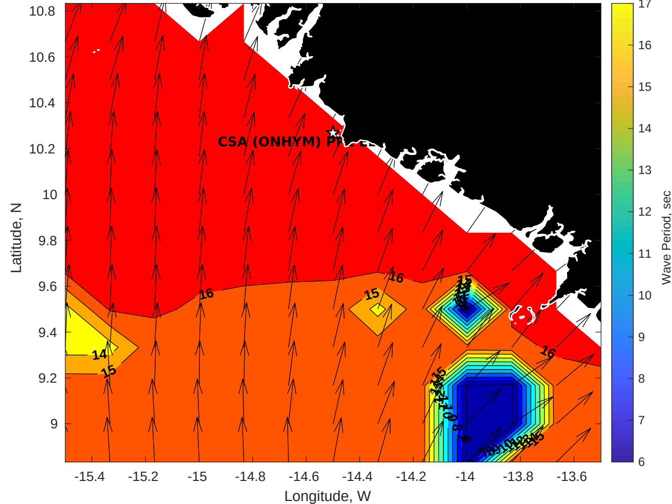
Wave Period (sec) for CSA (ONHYM) PPL EBS - Guinea at 08-Aug-2025 09:00:00
