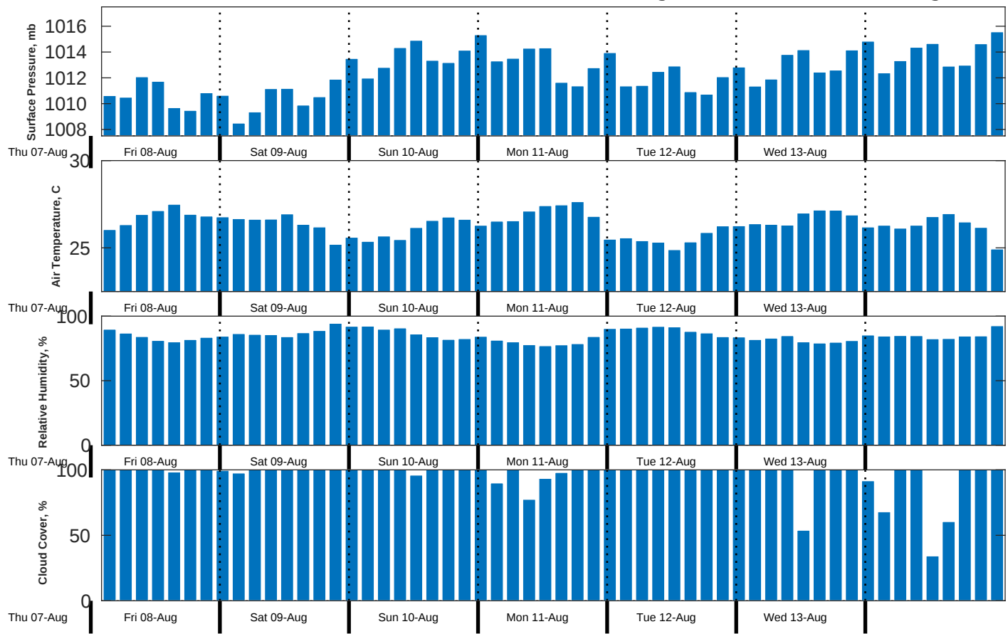
Met Forecast for CSA (ONHYM) PPL EBS - Guinea from 08-Aug-2025 00:00:00 to 15-Aug-2025 00:00:00
