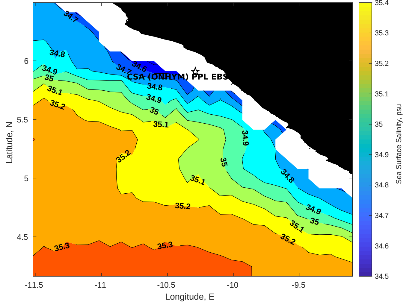
Surface Salinity for CSA (ONHYM) PPL EBS - Liberia at 07-Aug-2025 00:00:00
