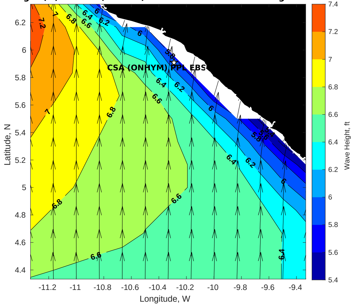
Wave Height (ft) for CSA (ONHYM) PPL EBS - Liberia at 08-Aug-2025 09:00:00
