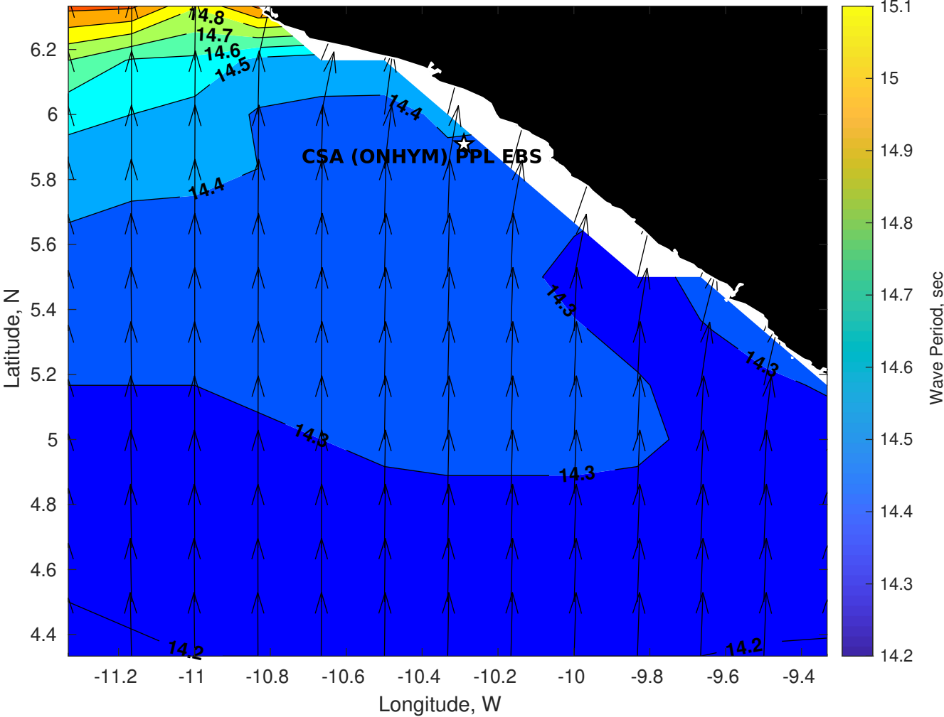
Wave Period (sec) for CSA (ONHYM) PPL EBS - Liberia at 08-Aug-2025 09:00:00
