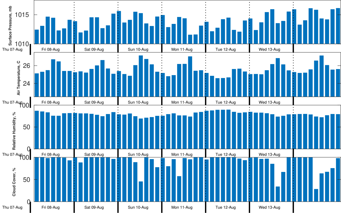
Met Forecast for CSA (ONHYM) PPL EBS - Liberia from 08-Aug-2025 00:00:00 to 15-Aug-2025 00:00:00
