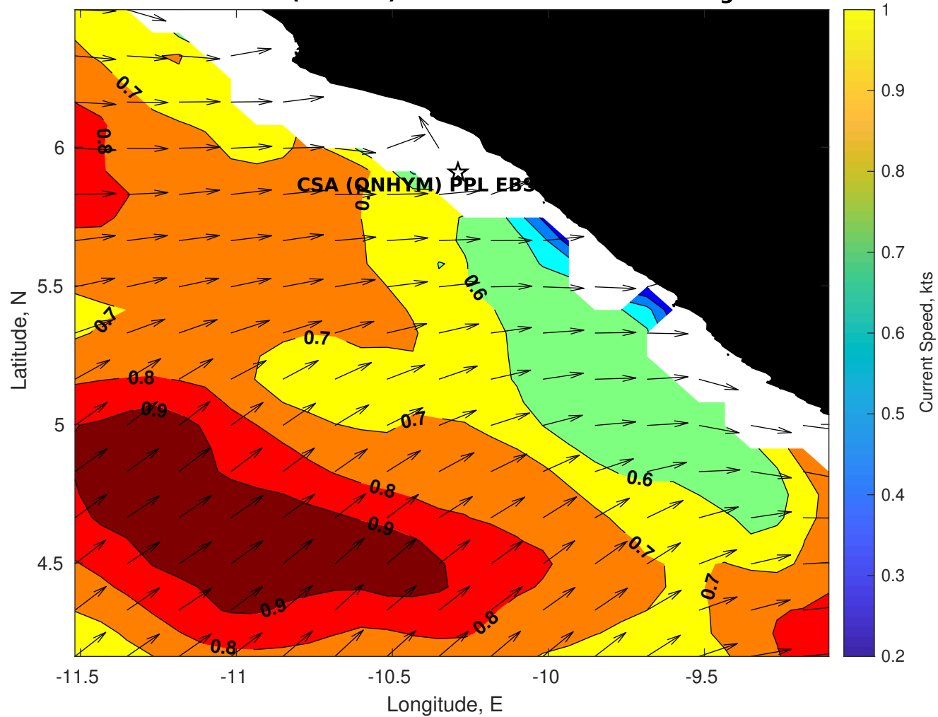
Surface Currents for CSA (ONHYM) PPL EBS - Liberia at 07-Aug-2025 00:00:00
