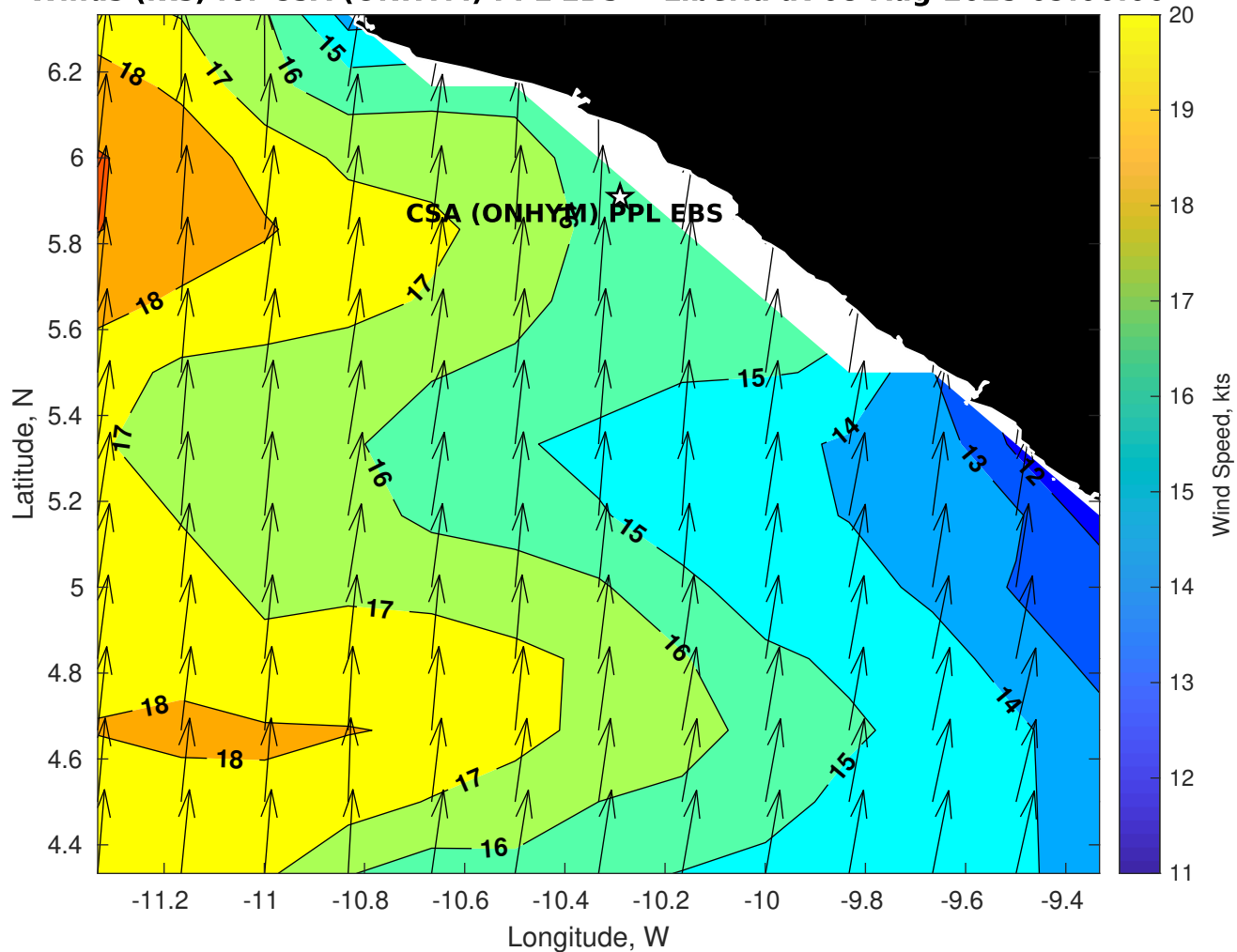
Winds (kts) for CSA (ONHYM) PPL EBS - Liberia at 08-Aug-2025 09:00:00
