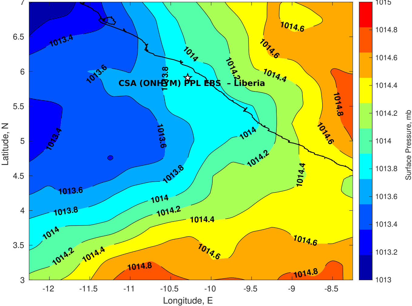
Surface Pressure (mb) for CSA (ONHYM) PPL EBS - Liberia at 09-Aug-2025 00:00:00
