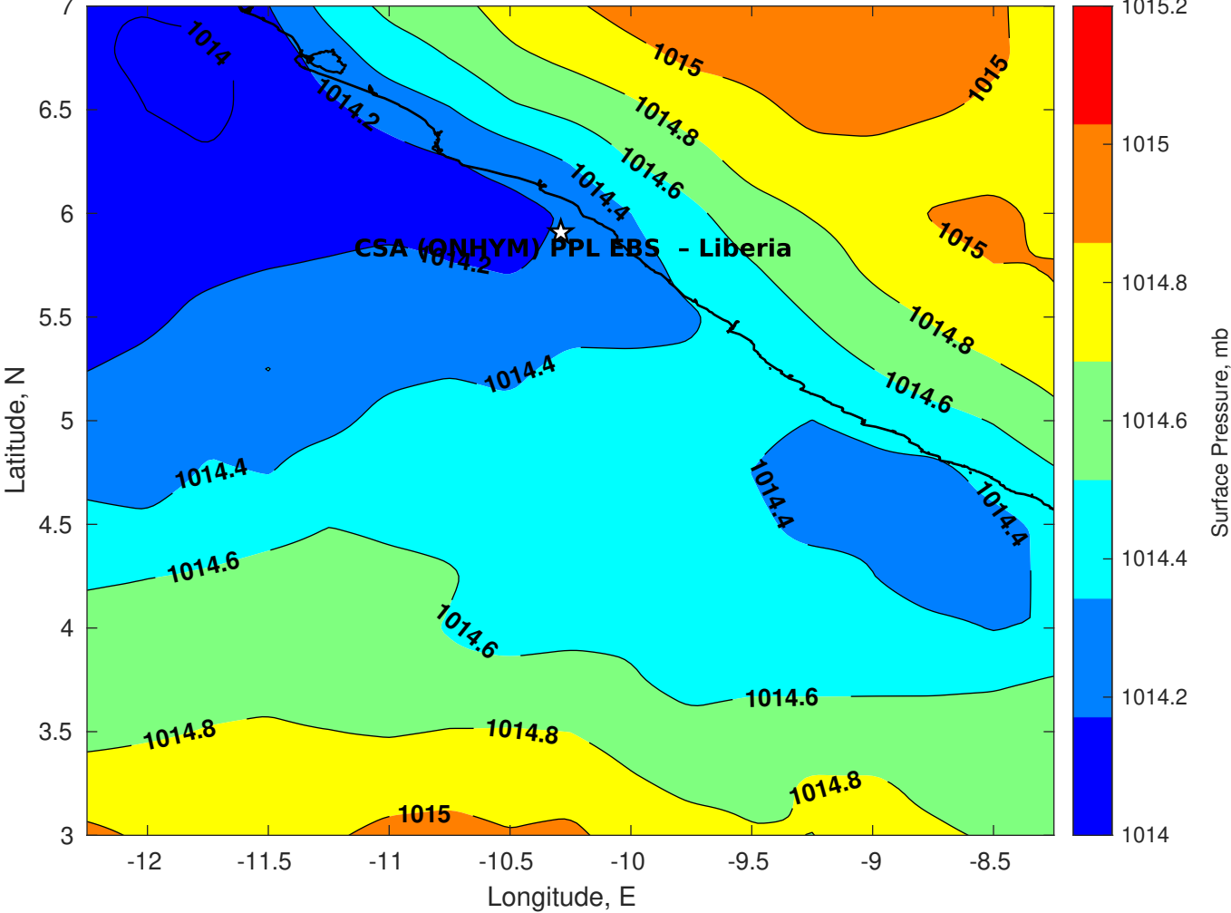
Surface Pressure (mb) for CSA (ONHYM) PPL EBS - Liberia at 08-Aug-2025 00:00:00
