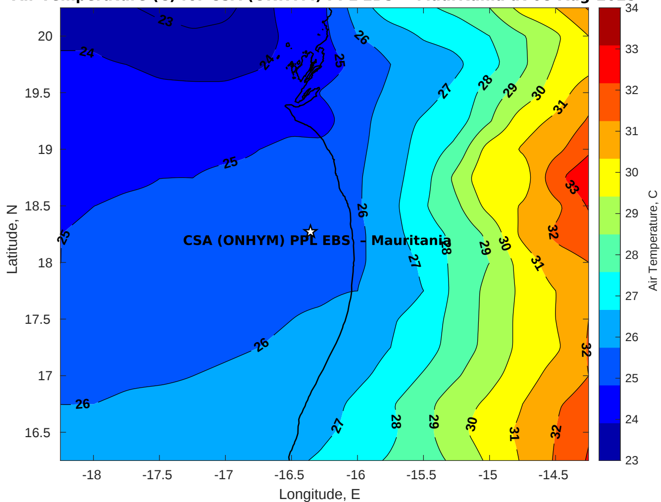
Air Temperature (C) for CSA (ONHYM) PPL EBS - Mauritania at 08-Aug-2025
