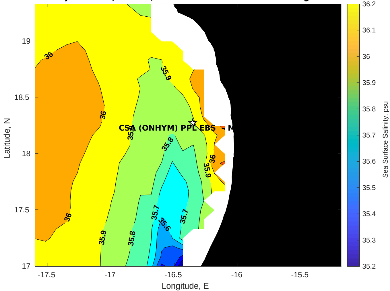
Surface Salinity for CSA (ONHYM) PPL EBS - Mauritania at 07-Aug-2025 00:00:00
