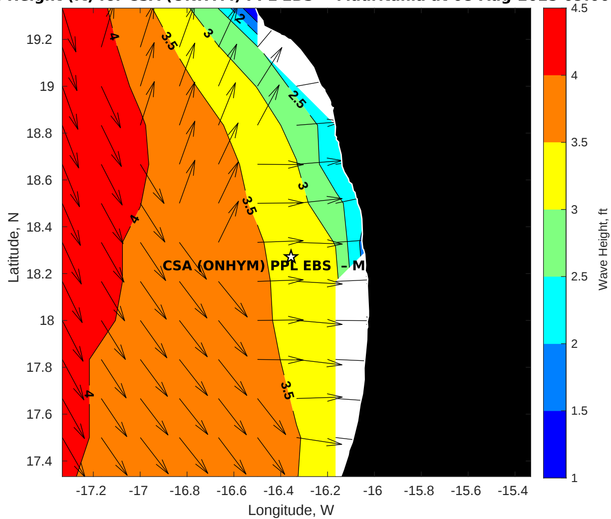
Wave Height (ft) for CSA (ONHYM) PPL EBS - Mauritania at 08-Aug-2025 09:00:00
