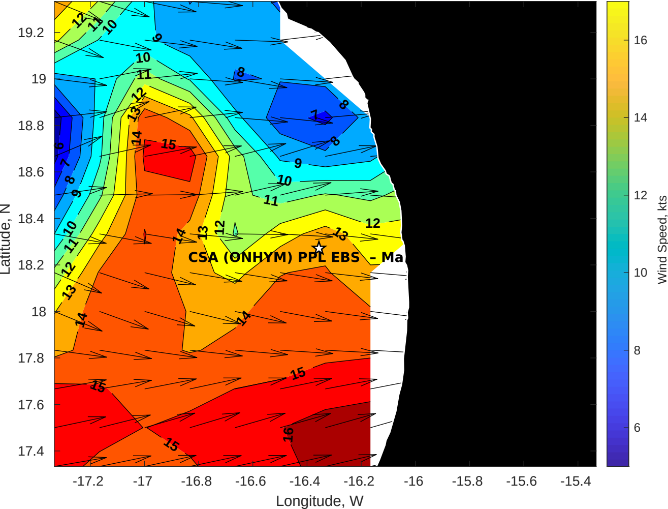
Winds (kts) for CSA (ONHYM) PPL EBS - Mauritania at 08-Aug-2025 09:00:00
