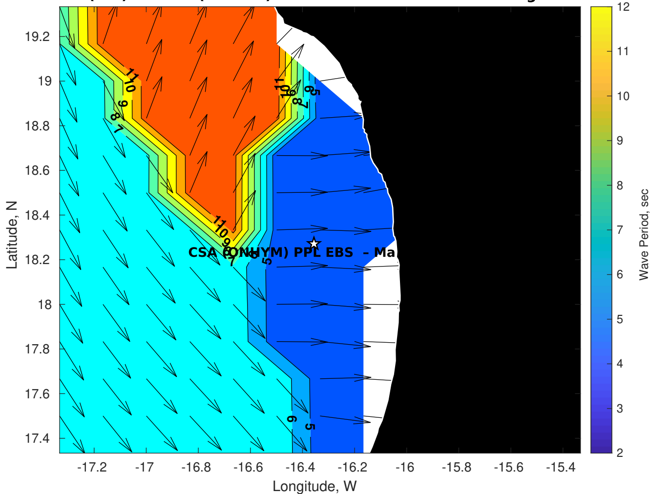
Wave Period (sec) for CSA (ONHYM) PPL EBS - Mauritania at 08-Aug-2025 09:00:00
