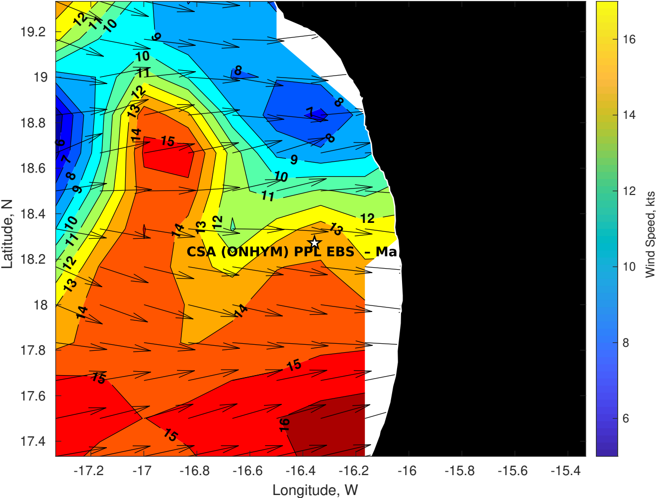
Winds (kts) for CSA (ONHYM) PPL EBS - Mauritania at 08-Aug-2025 09:00:00
