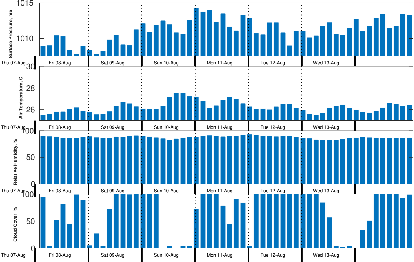
Met Forecast for CSA (ONHYM) PPL EBS - Mauritania from 08-Aug-2025 00:00:00 to 15-Aug-2025 00:00:00
