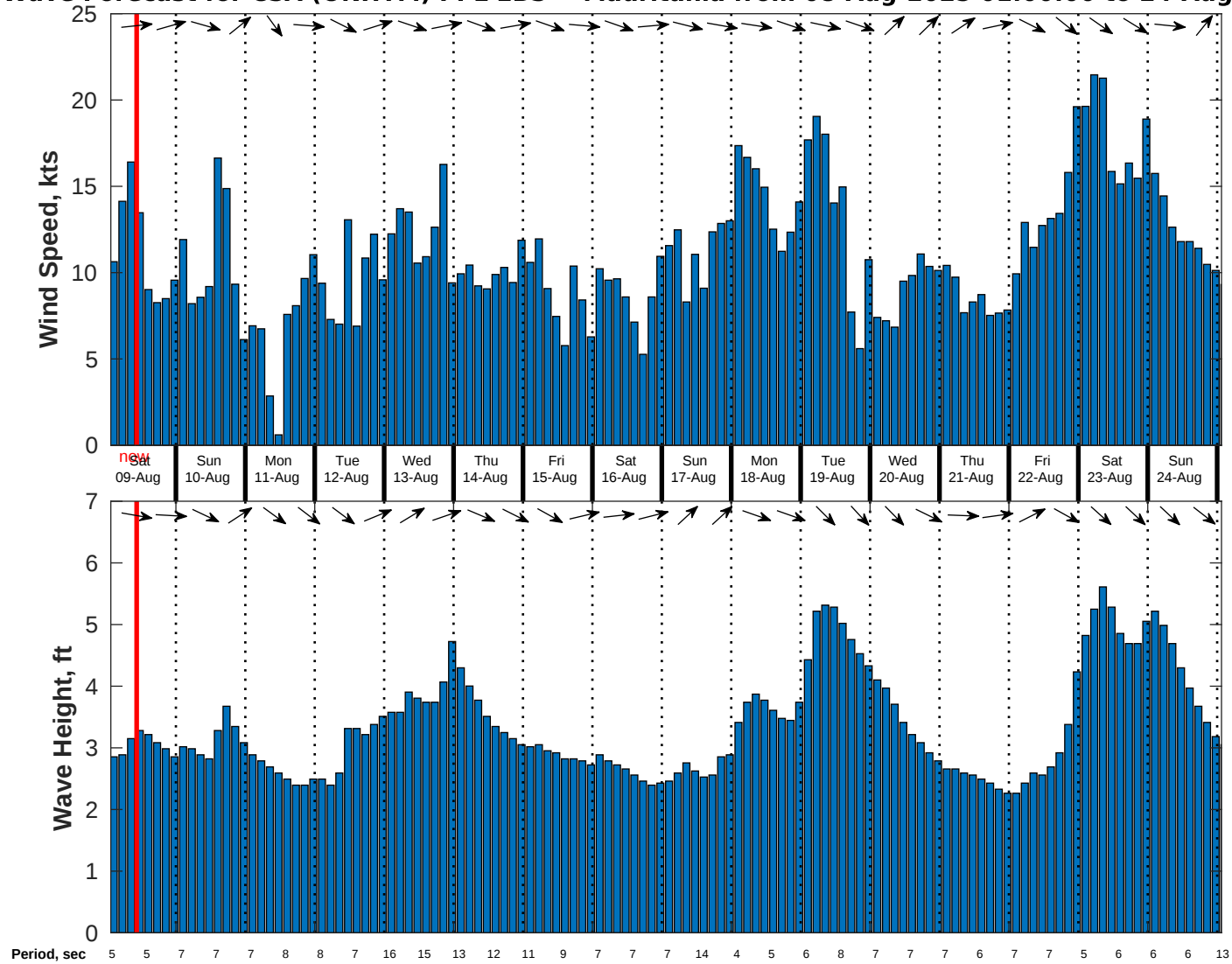
Wind & Wave Forecast for CSA (ONHYM) PPL EBS - Mauritania from 08-Aug-2025 01:00:00 to 24-Aug-2025 01:00:00
