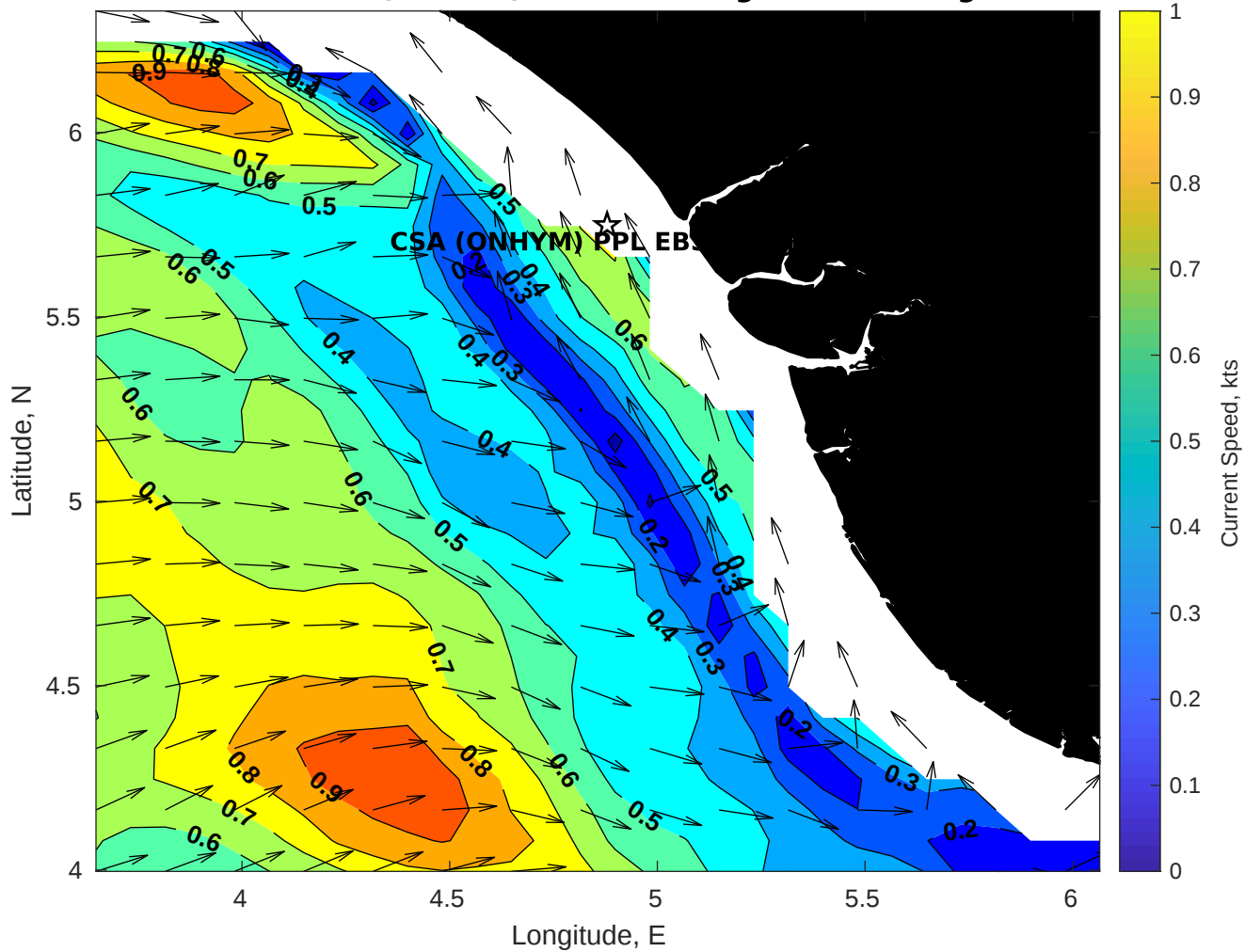
Surface Currents for CSA (ONHYM) PPL EBS - Nigeria at 07-Aug-2025 00:00:00
