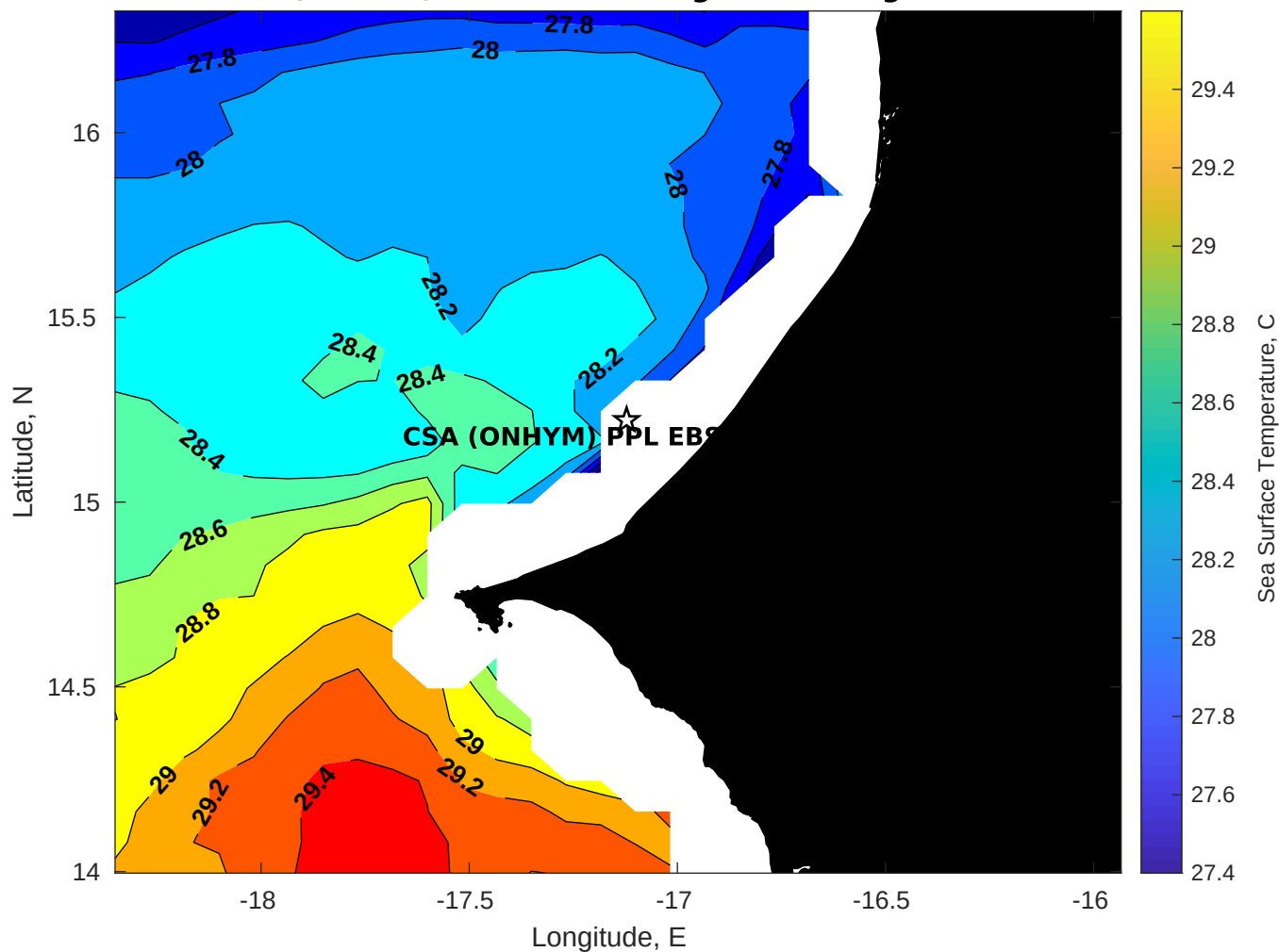
SST for CSA (ONHYM) PPL EBS - Senegal at 07-Aug-2025 00:00:00
