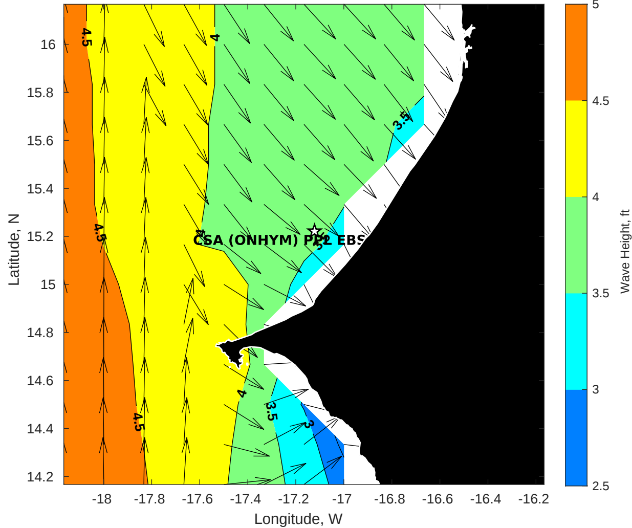
Wave Height (ft) for CSA (ONHYM) PPL EBS - Senegal at 08-Aug-2025 09:00:00
