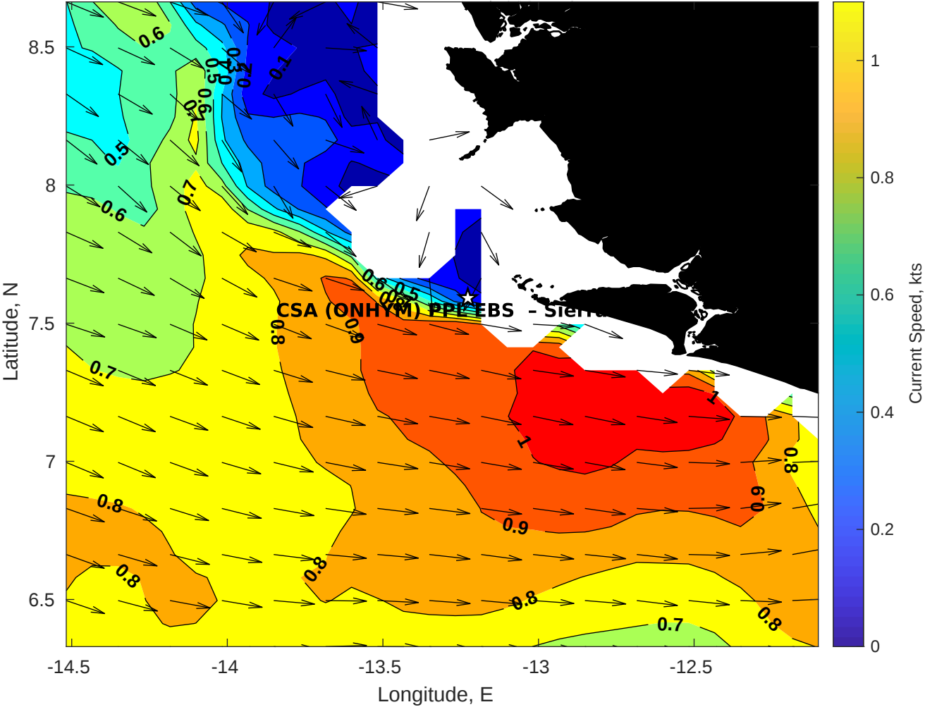
Surface Currents for CSA (ONHYM) PPL EBS - Sierra Leone at 07-Aug-2025 00:00:00
