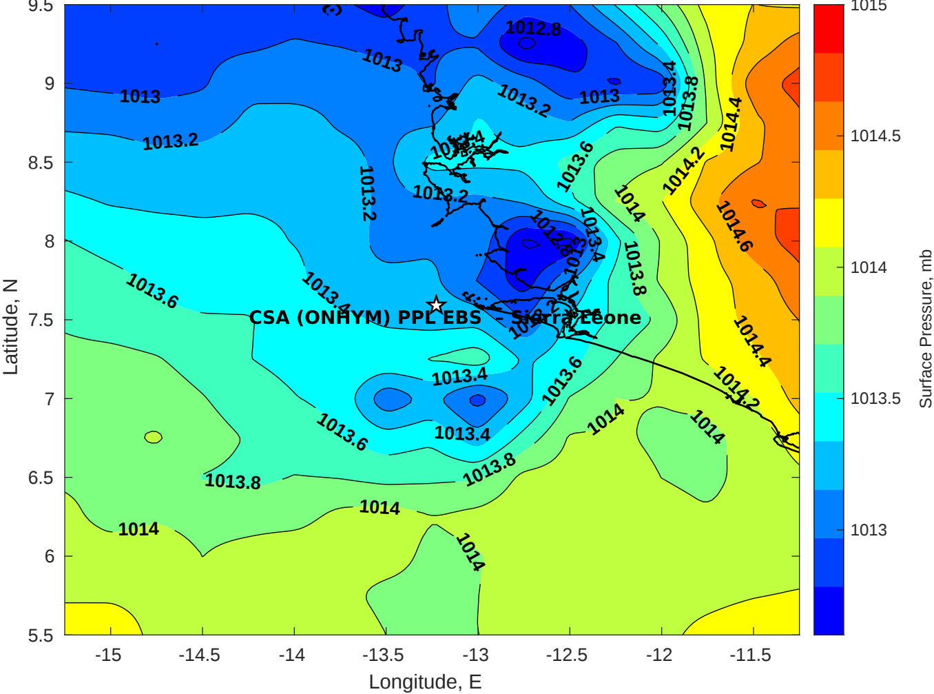
Surface Pressure (mb) for CSA (ONHYM) PPL EBS - Sierra Leone at 08-Aug-2025 00:00:00
