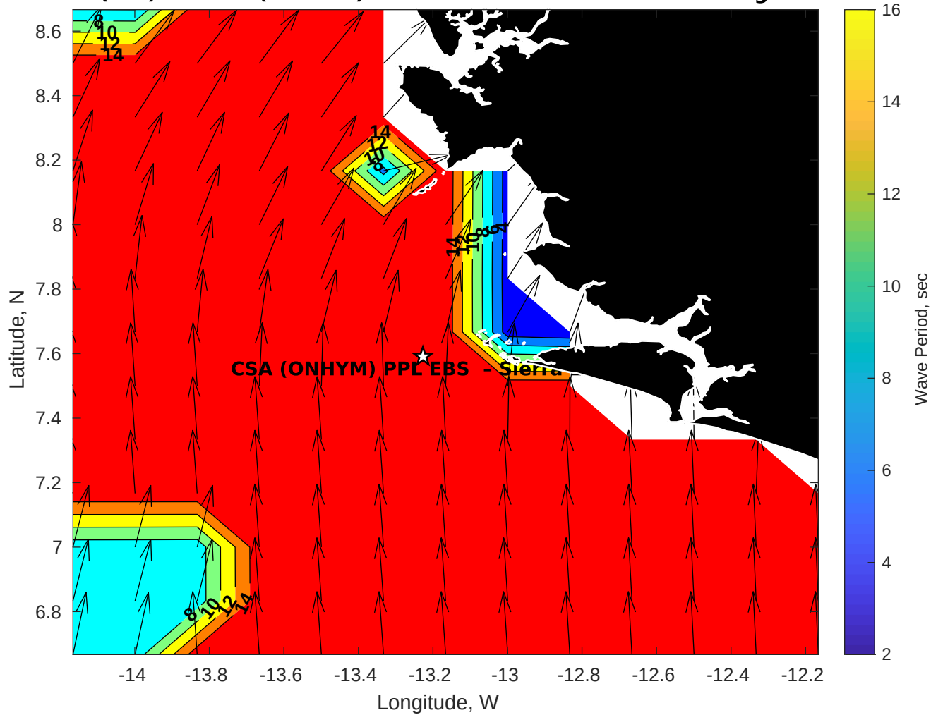
Wave Period (sec) for CSA (ONHYM) PPL EBS - Sierra Leone at 08-Aug-2025 09:00:00
