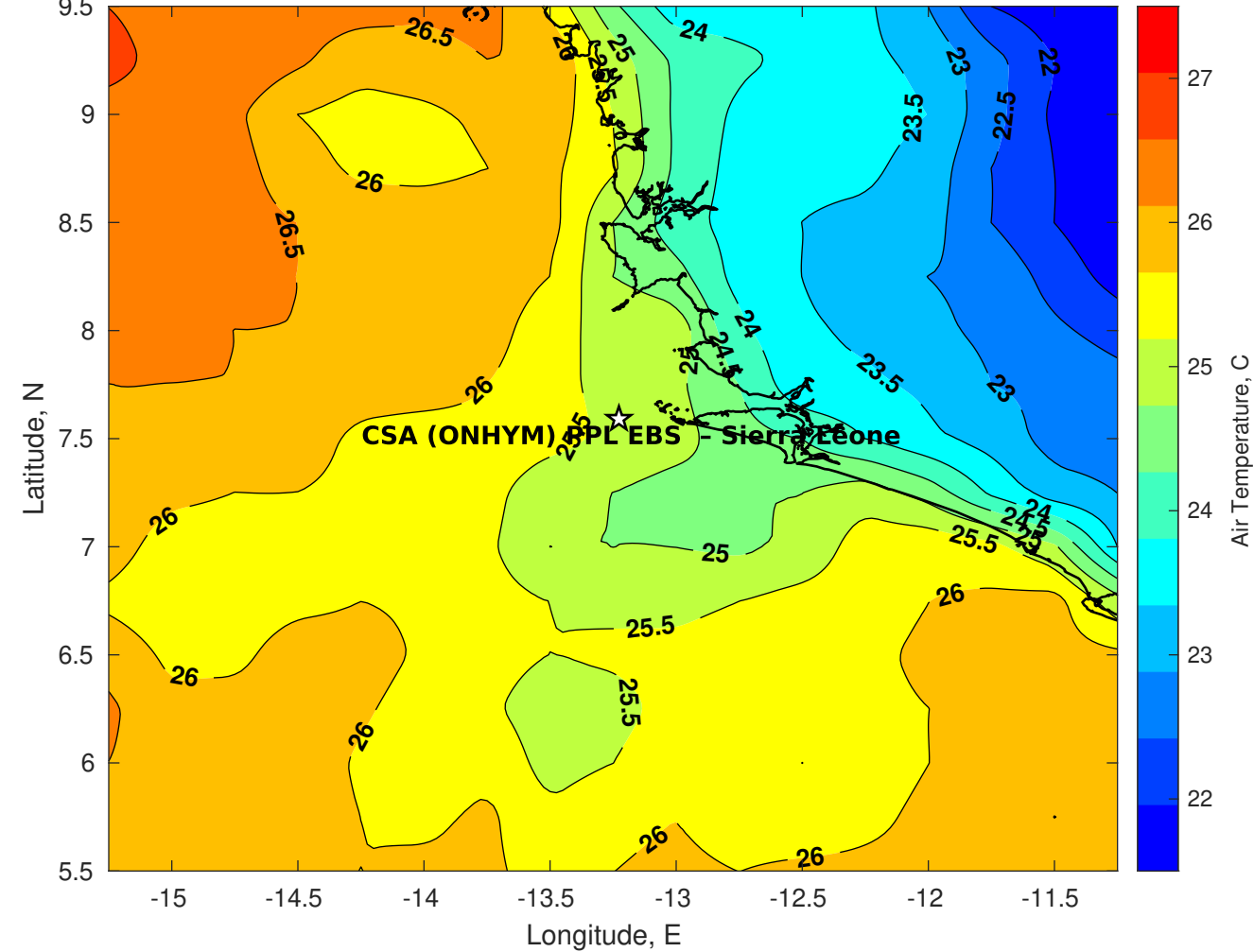
Air Temperature (C) for CSA (ONHYM) PPL EBS - Sierra Leone at 08-Aug-2025
