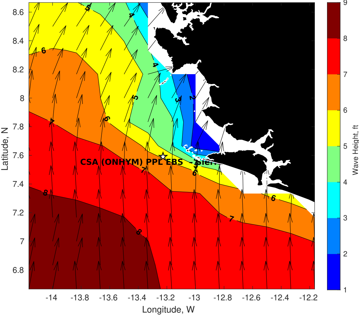
Wave Height (ft) for CSA (ONHYM) PPL EBS - Sierra Leone at 08-Aug-2025 09:00:00
