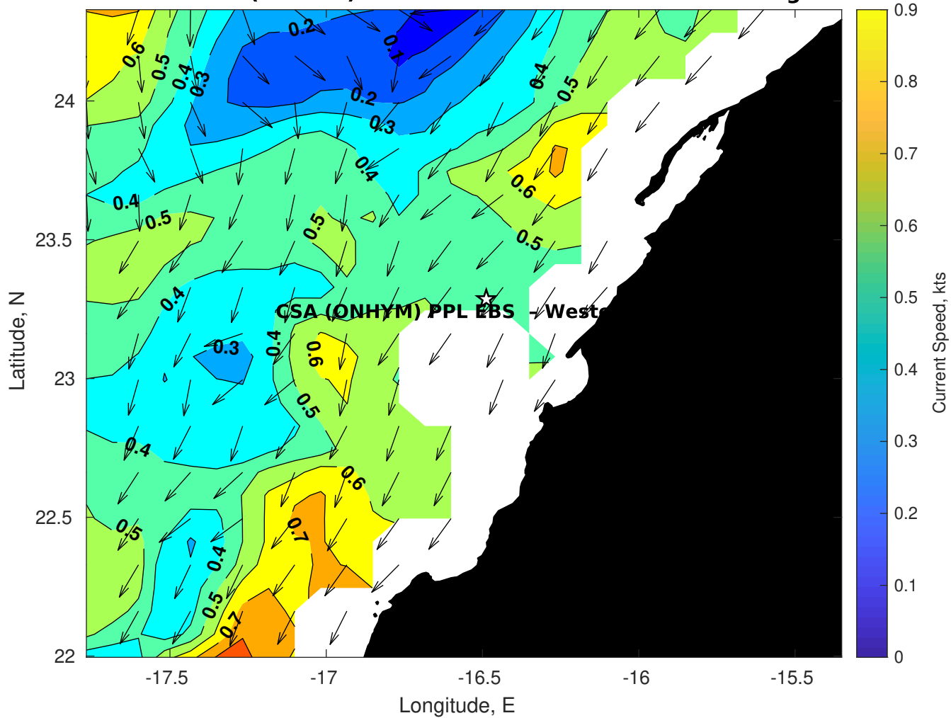
Surface Currents for CSA (ONHYM) PPL EBS - Western Sahara at 07-Aug-2025 00:00:00
