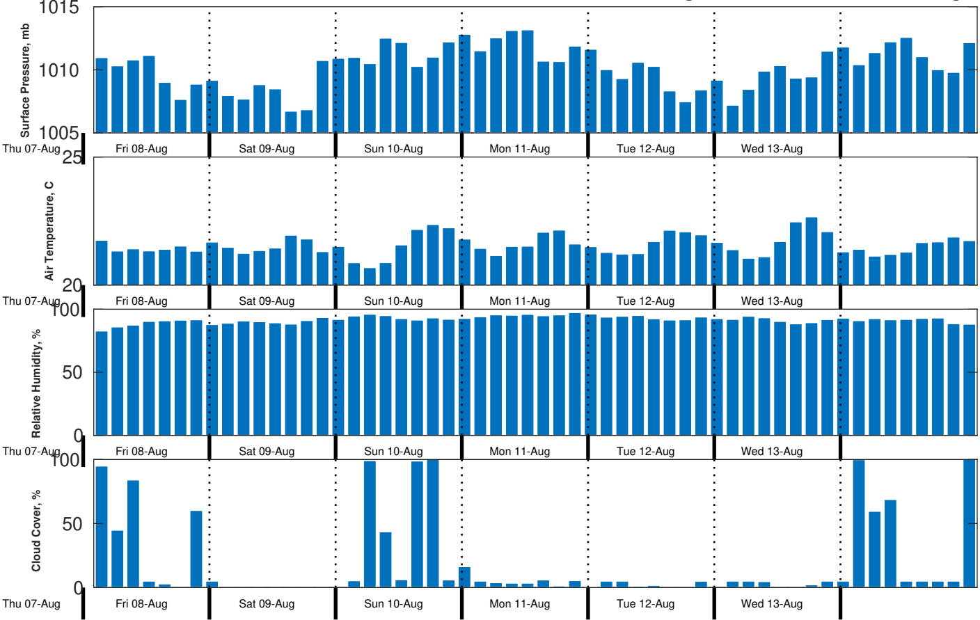
Met Forecast for CSA (ONHYM) PPL EBS - Western Sahara from 08-Aug-2025 00:00:00 to 15-Aug-2025 00:00:00
