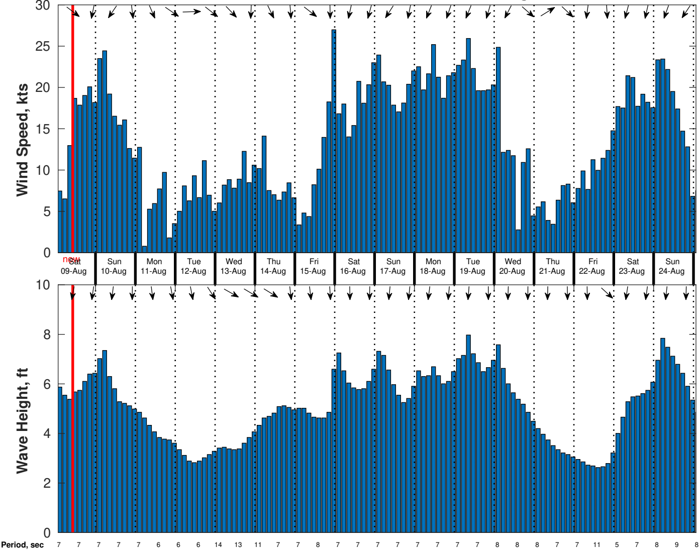
Wind & Wave Forecast for CSA (ONHYM) PPL EBS - Western Sahara from 08-Aug-2025 01:00:00 to 24-Aug-2025 01:00:00
