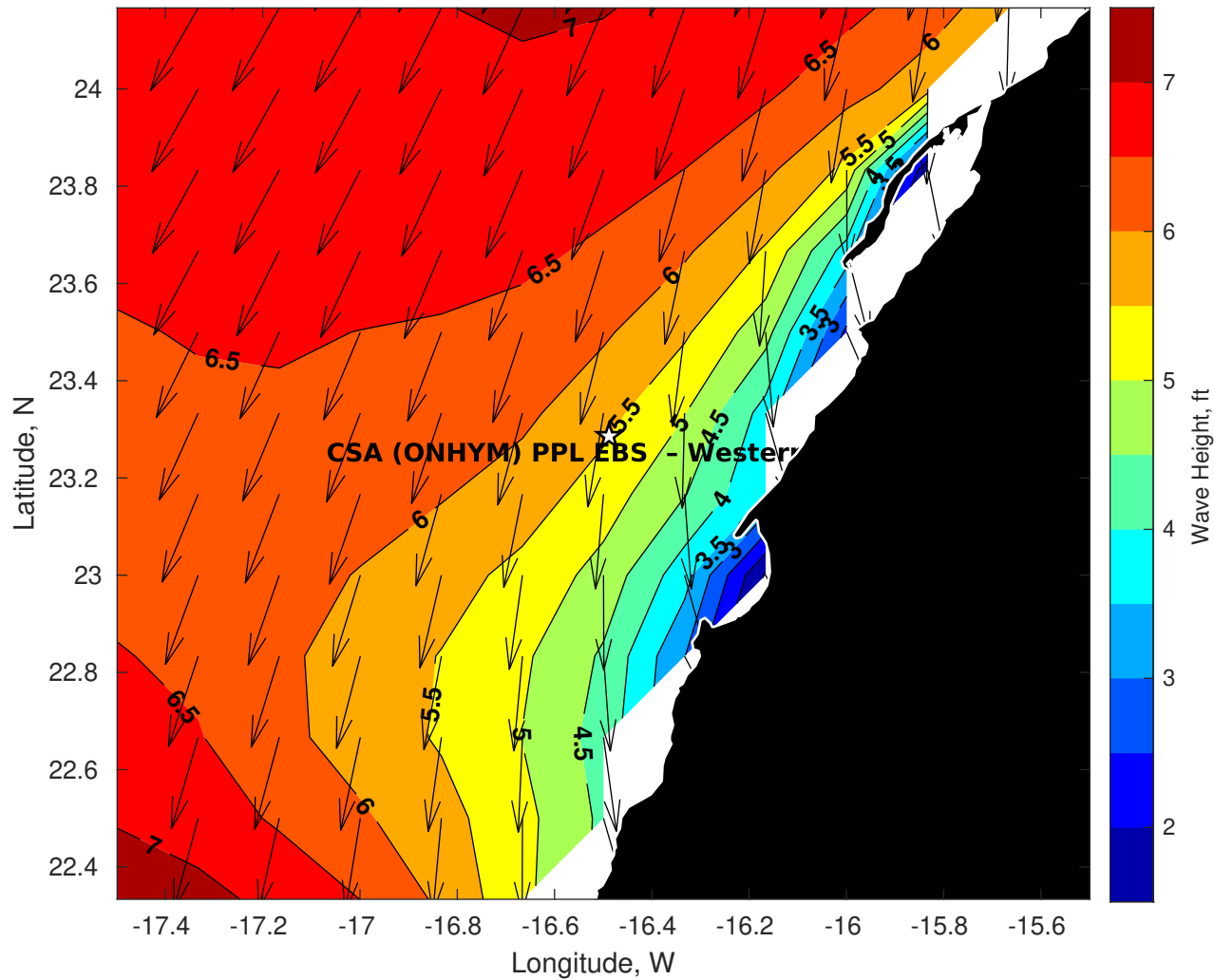
Wave Height (ft) for CSA (ONHYM) PPL EBS - Western Sahara at 08-Aug-2025 09:00:00
