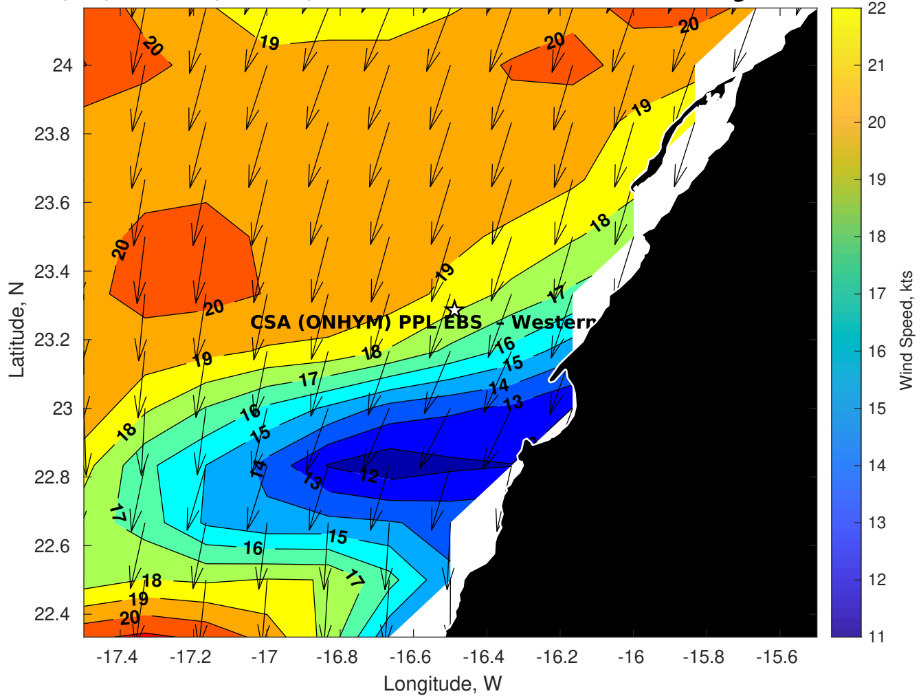
Winds (kts) for CSA (ONHYM) PPL EBS - Western Sahara at 08-Aug-2025 09:00:00
