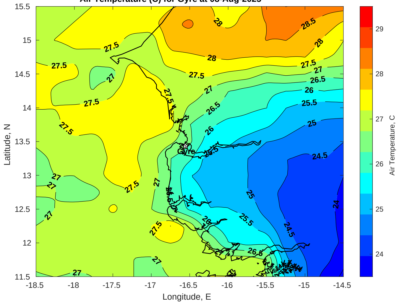
Air Temperature (C) for Gyre at 08-Aug-2025
